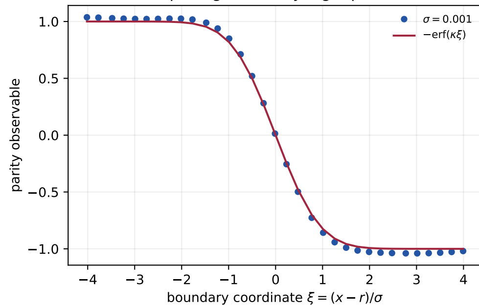
Repelling-boundary eigenprofile
