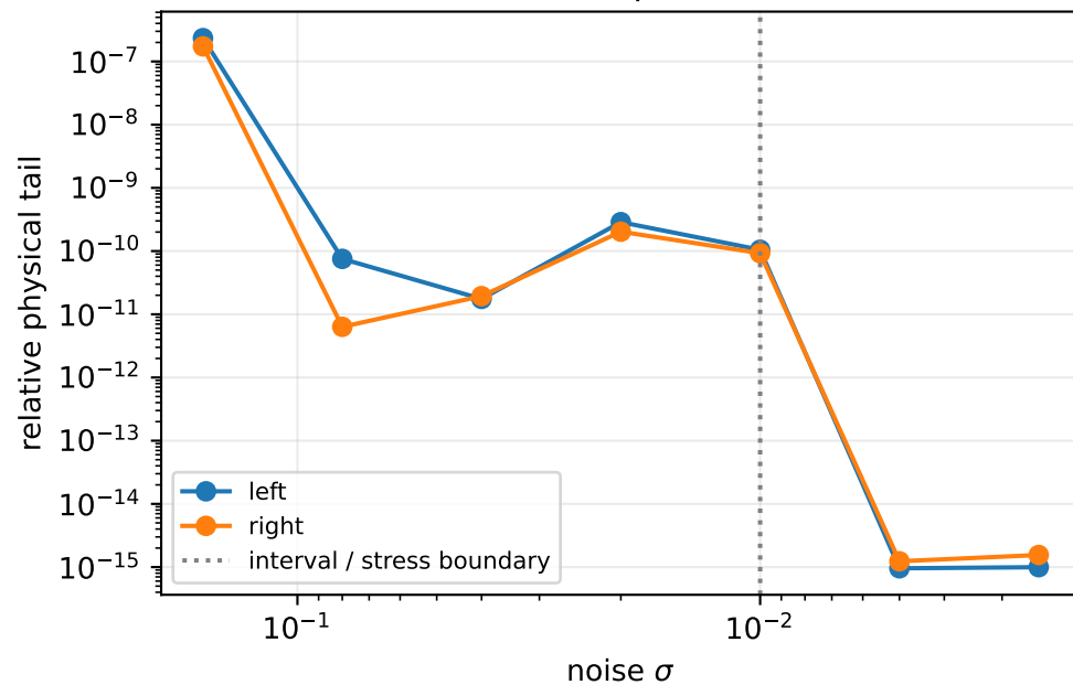
(b) Five interval scales plus two stress scales
