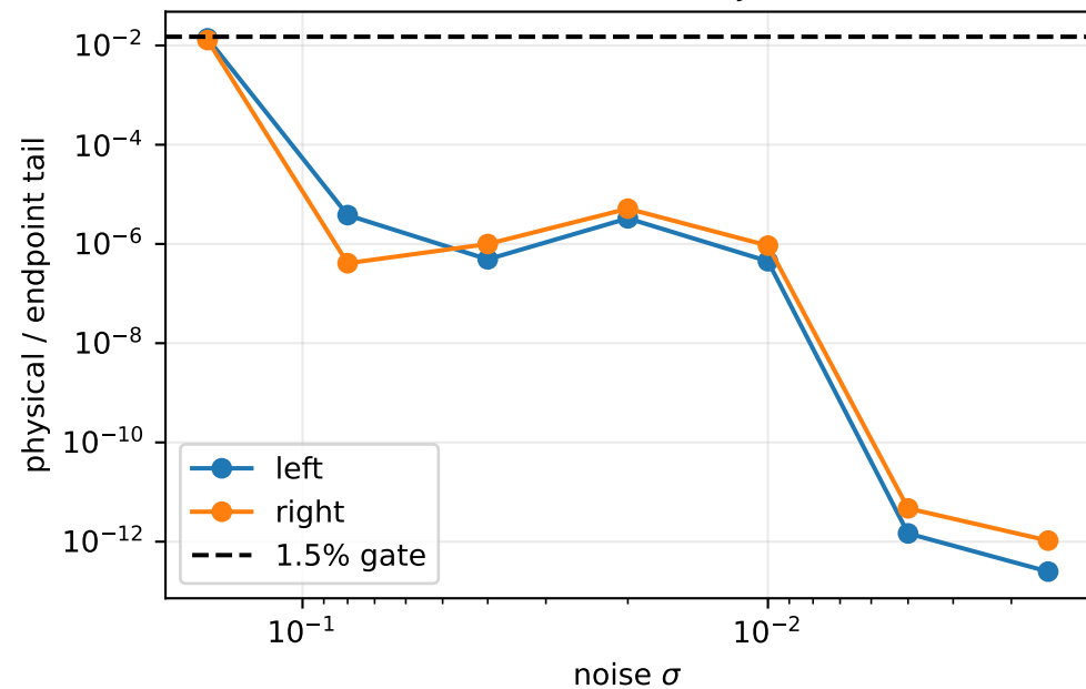
(a) Clock-rank tail majorization
