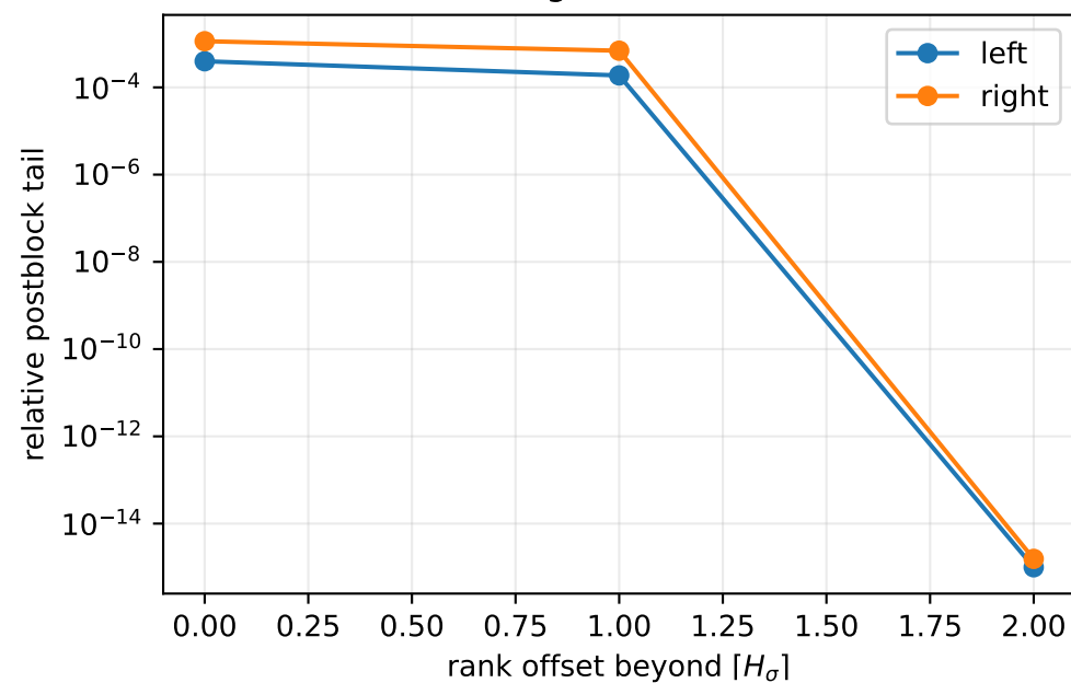
(c) Offset gain at \sigma = 0.0025
