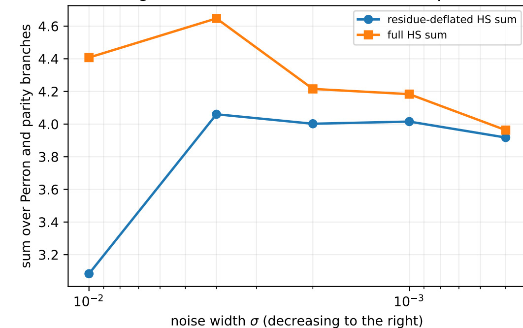
(c) Eight-node Hilbert--Schmidt directional plateau
