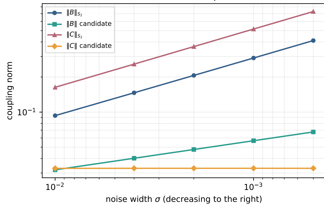
(a) Exact Haar Frobenius and operator candidates
