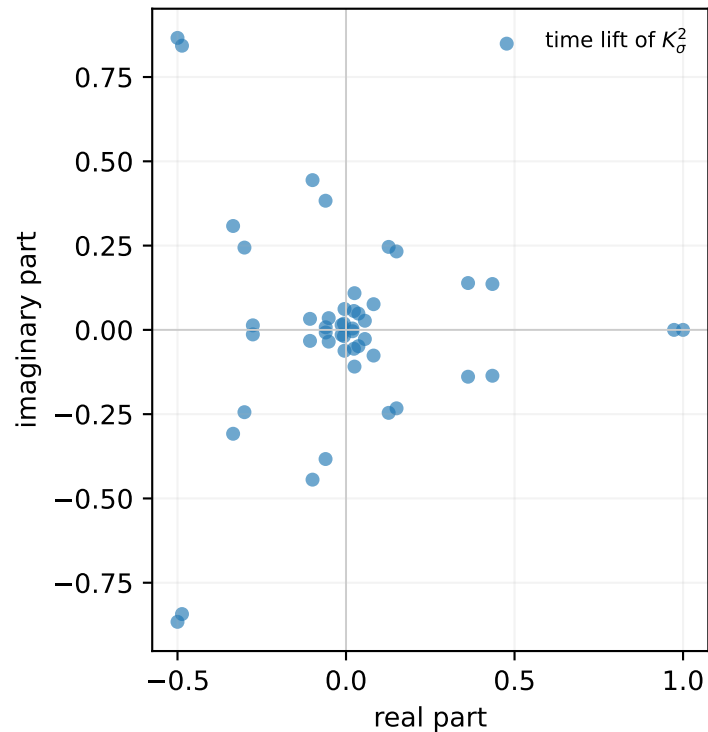
Exact Floquet replication
