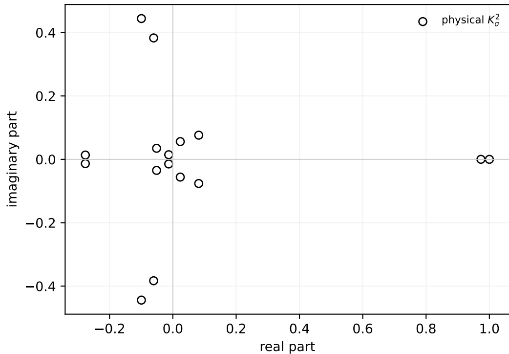
Physical two-step spectrum
