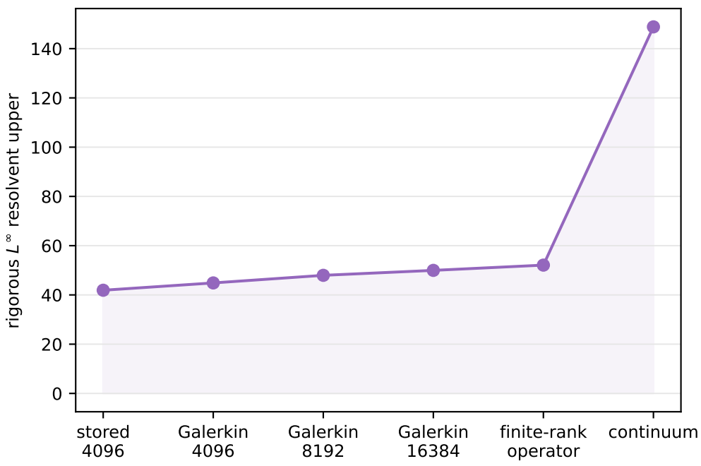
(c) Resolvent control survives the continuum lift
