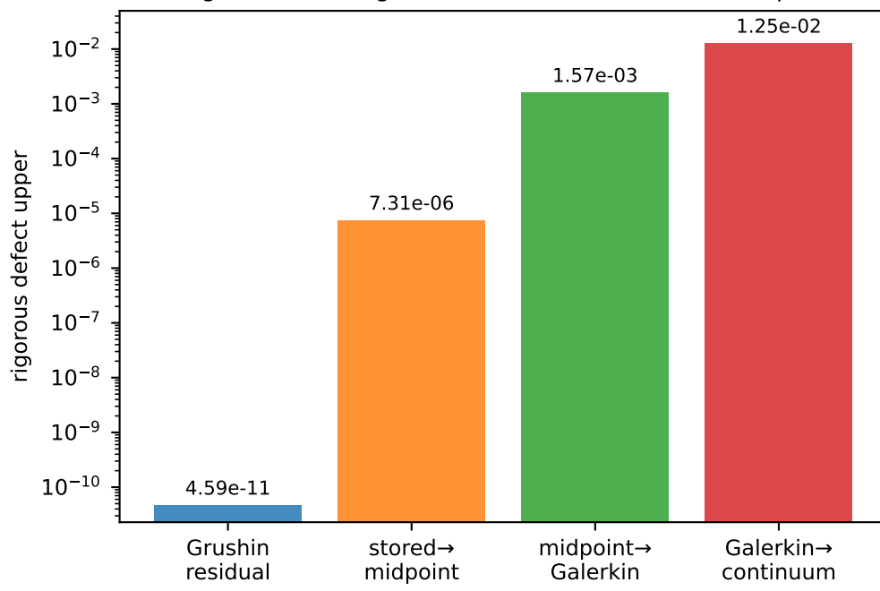
(d) Algebraic, finite-grid, and continuum errors are separated
