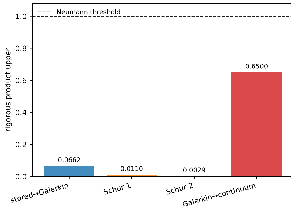
(d) Algebraic, finite-grid, and continuum errors are separated
