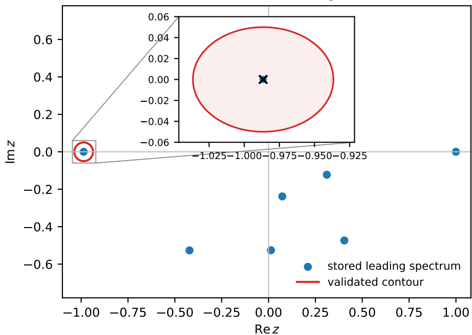
(a) A certified circle isolates the negative resonance
