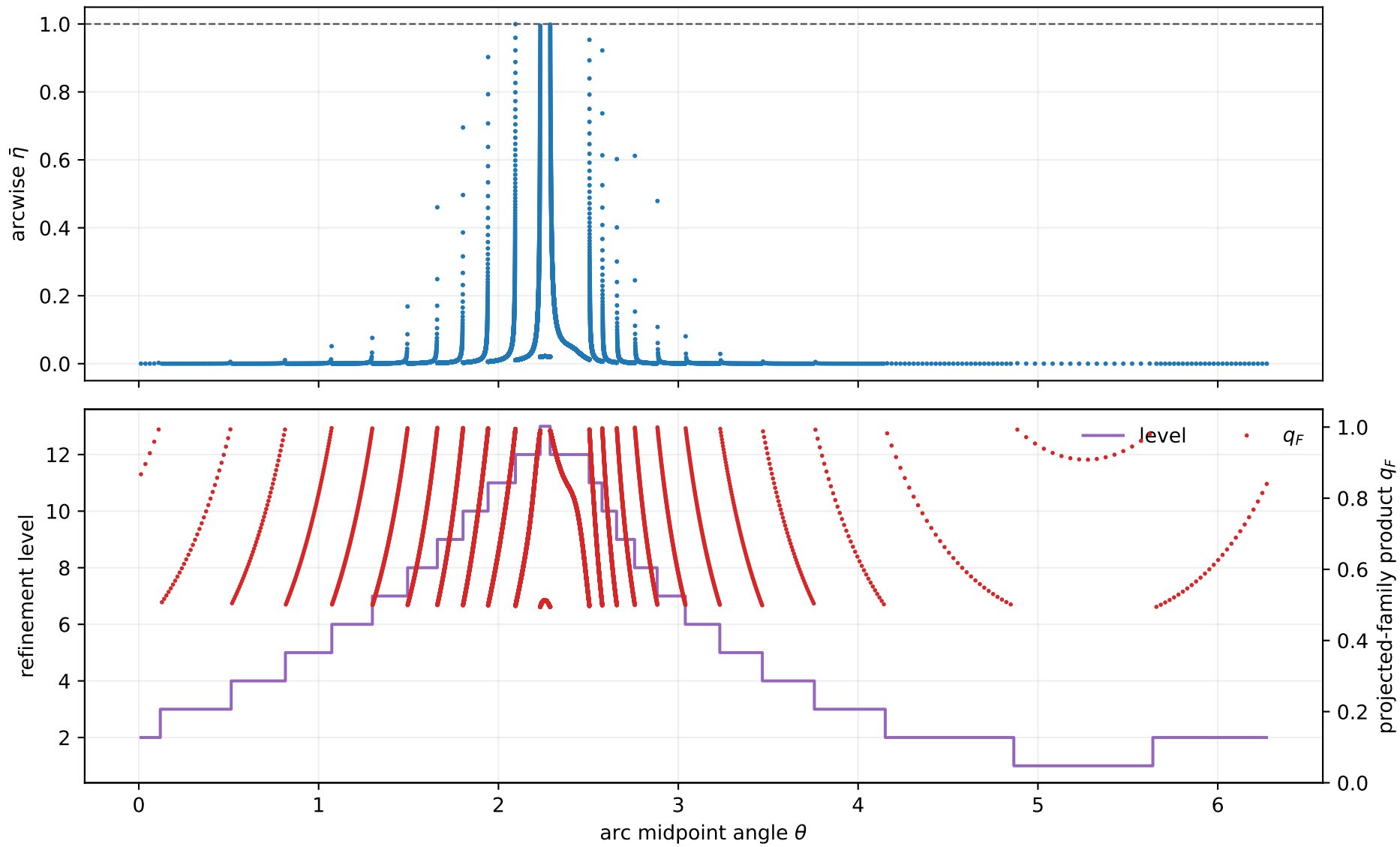
Adaptive full-contour cover, \sigma = 1e-04
