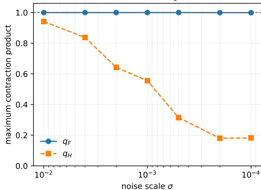
Local Neumann gates
