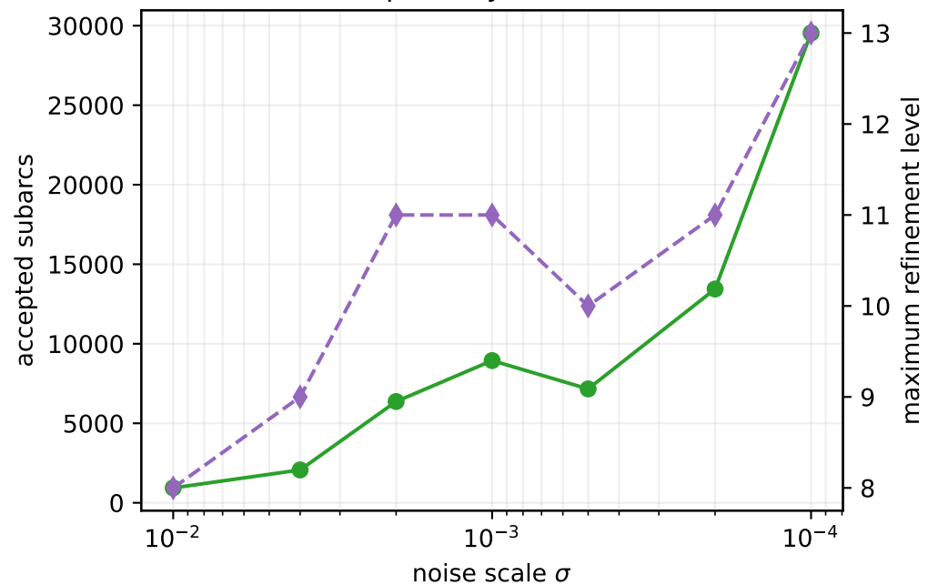
Adaptive dyadic cover
