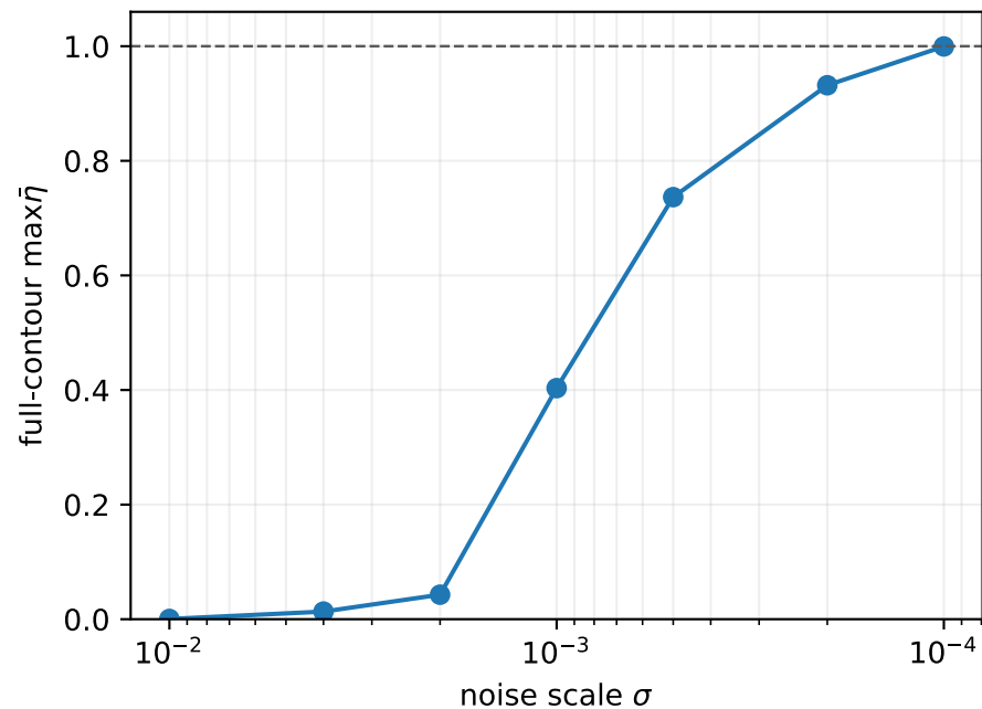
Conditional Rouché ratio
