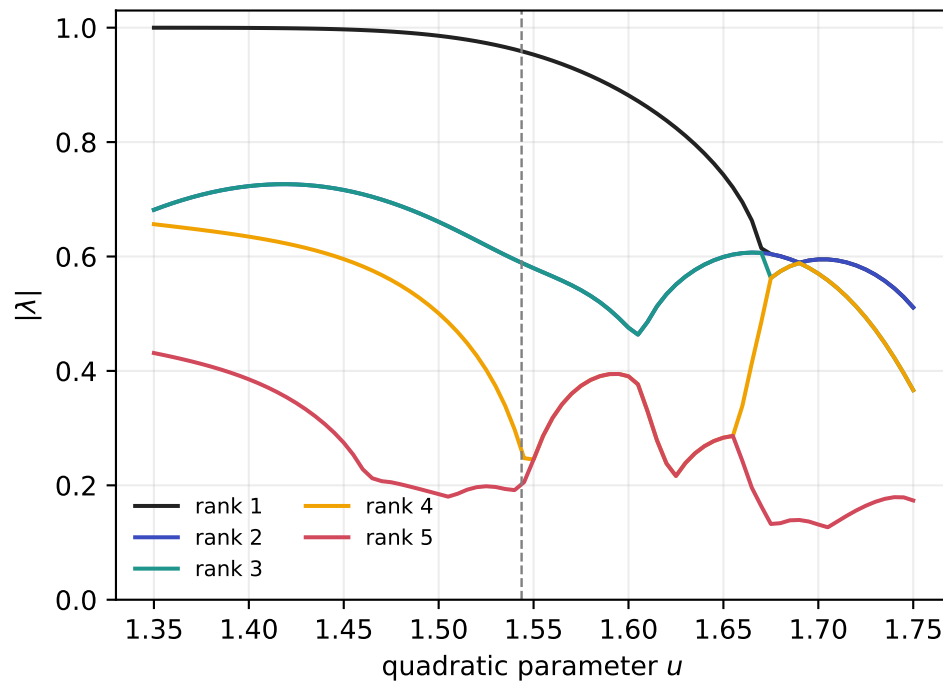
Ordered resonance moduli, \sigma = 0.05
