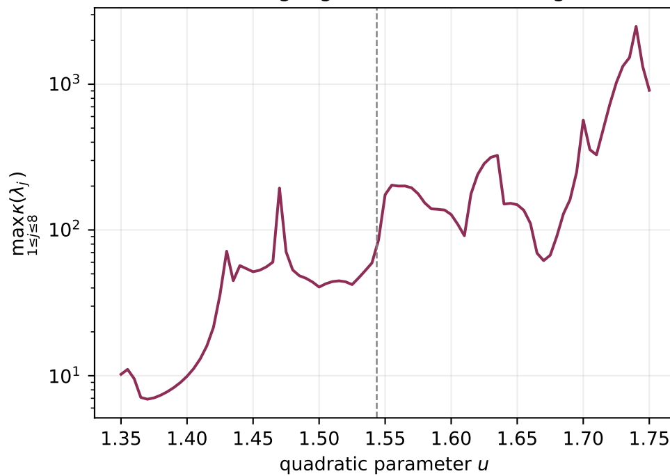
Leading eigenvalue conditioning
