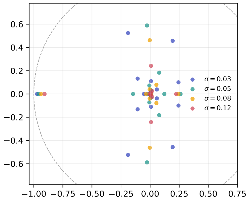
Non-Perron spectrum at u_c
