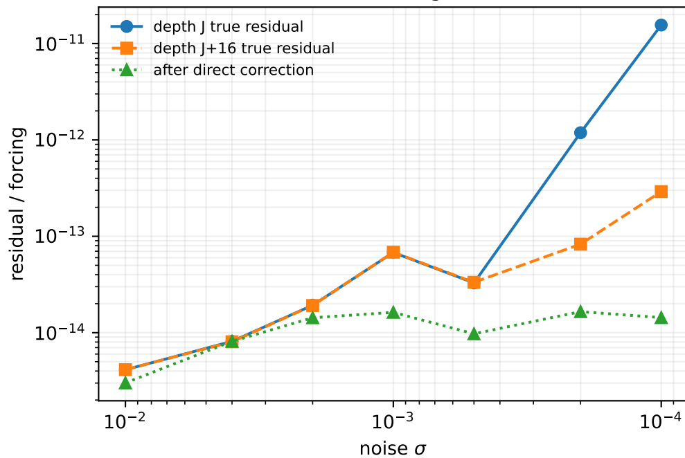
Ambient residuals, including recurrence defects
