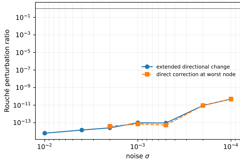
Direct low-rank correction confirms the extension
