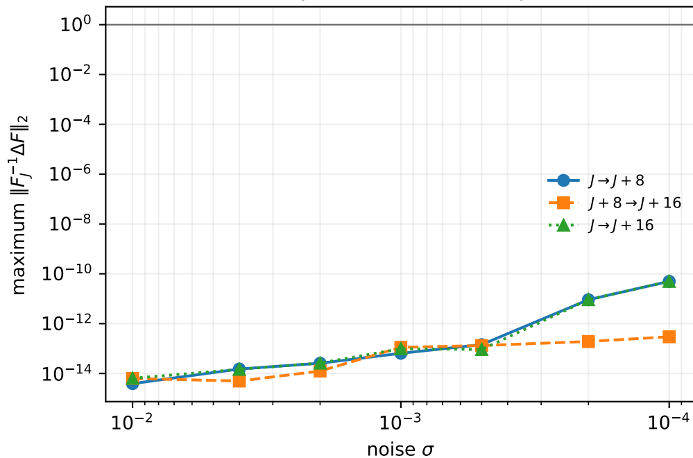
Directional Krylov increments stay below one
