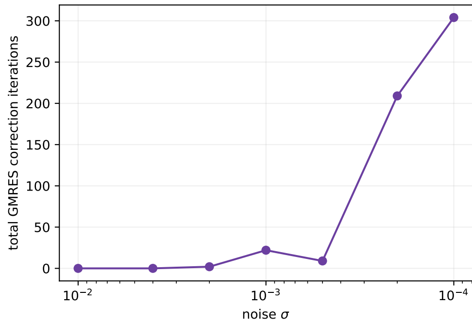
Direct directional closure becomes costlier
