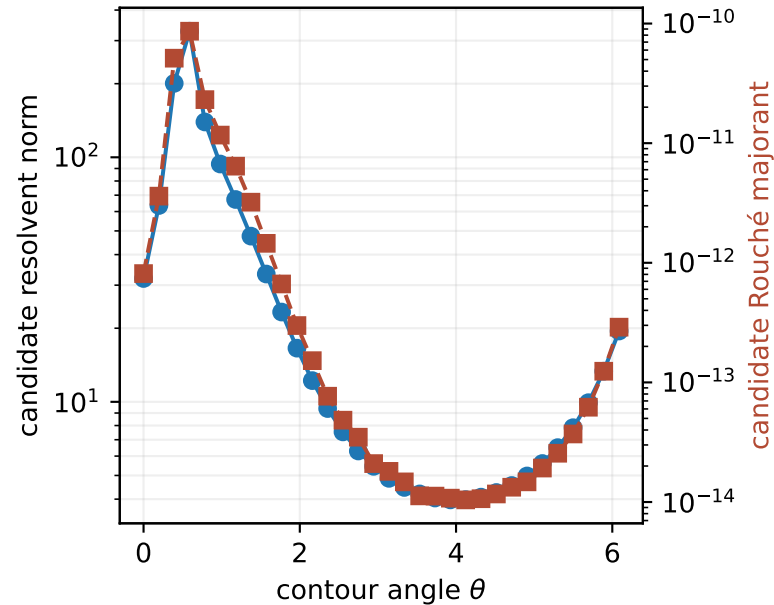
Global scalar route at \sigma = 10^{-2}
