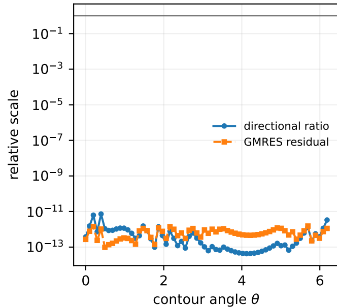
Direct full-Feshbach cross-check
