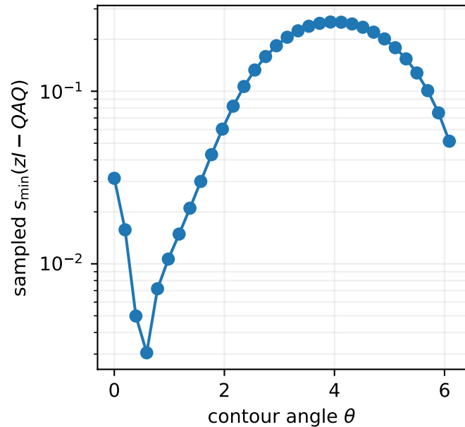
Global singular-value candidates
