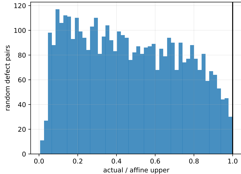
One-step theorem efficiency
