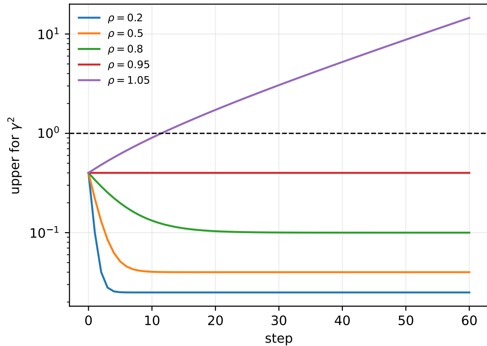
Affine recurrence regimes
