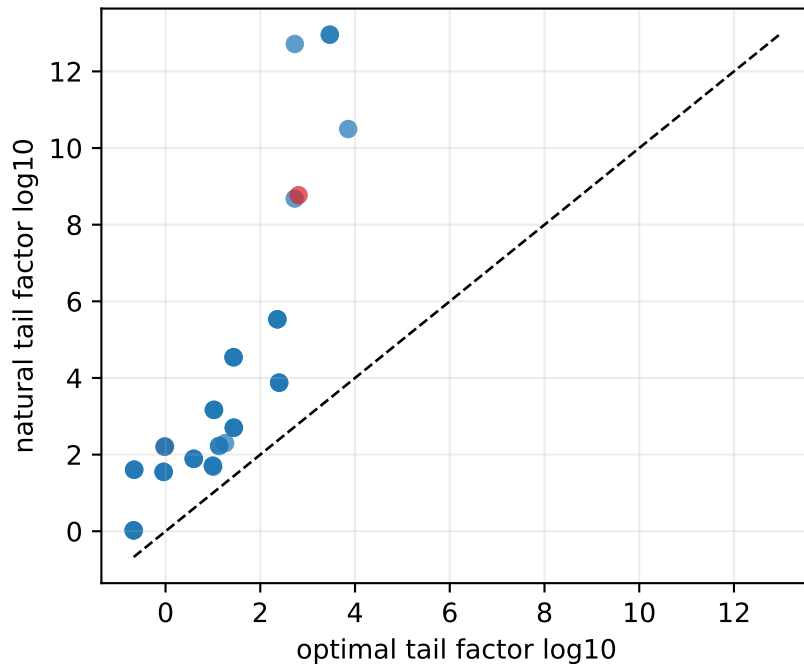
Exact-Gram lift is feasible but nonoptimal
