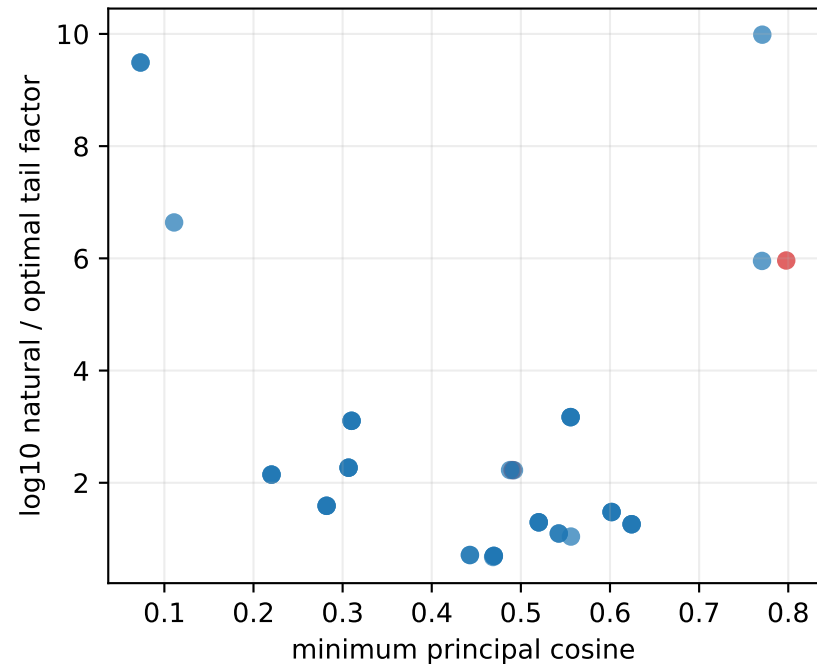
Packet angle does not control tail alignment
