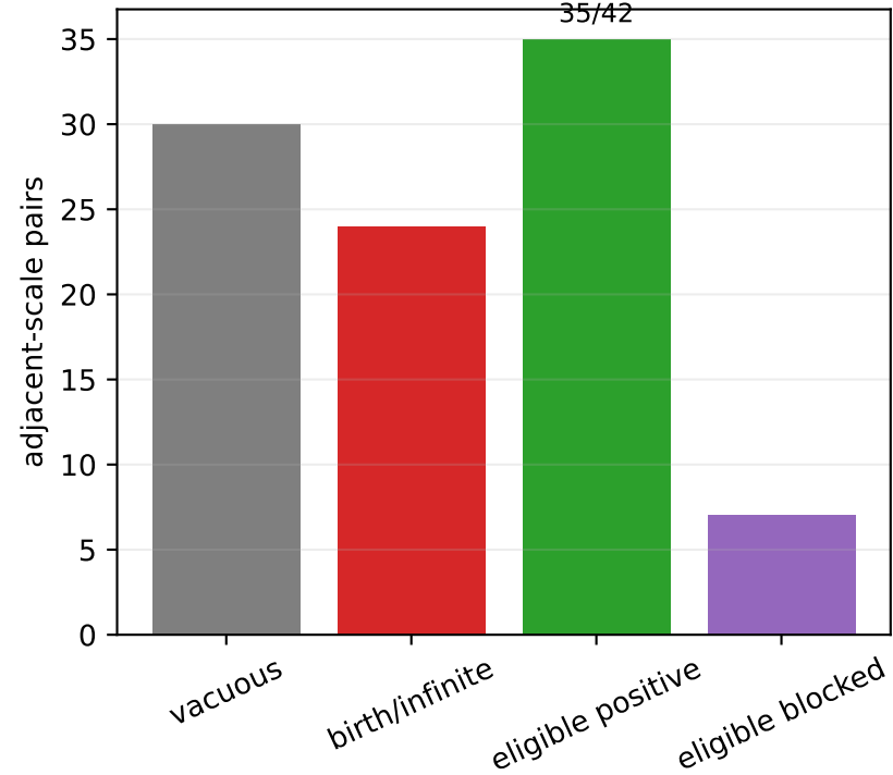
Natural dyadic-gauge outcome
