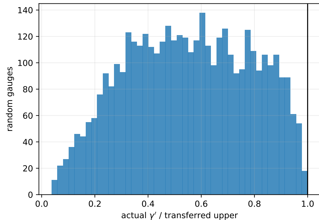
Relative-tail transfer
