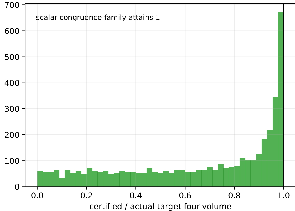
Determinant transfer
