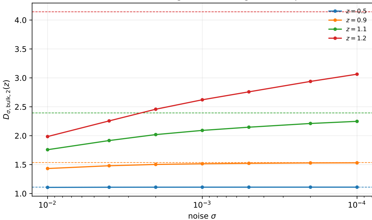
Coefficientwise target and slowing near the pole
