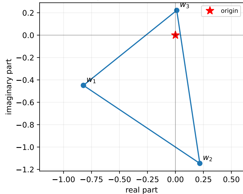
Certified compressed numerical-range witness
