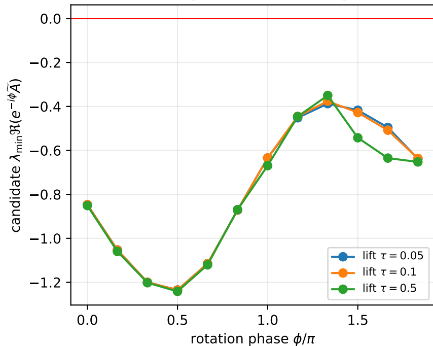
Accretivity scan remains negative
