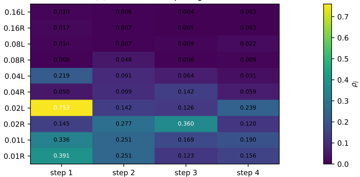
(b) Variable one-step budgets
