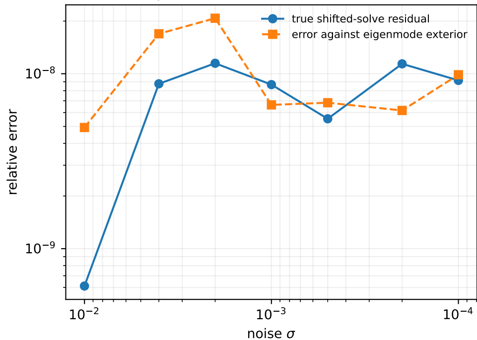
Independent resolvent reconstruction
