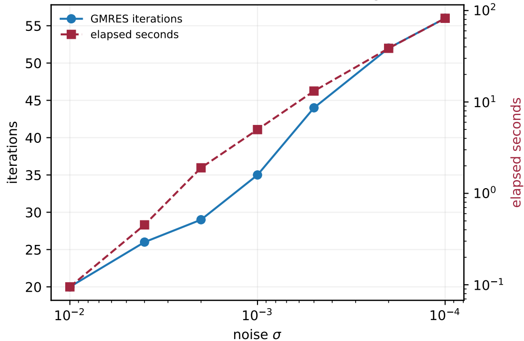
The shifted solve remains convergent
