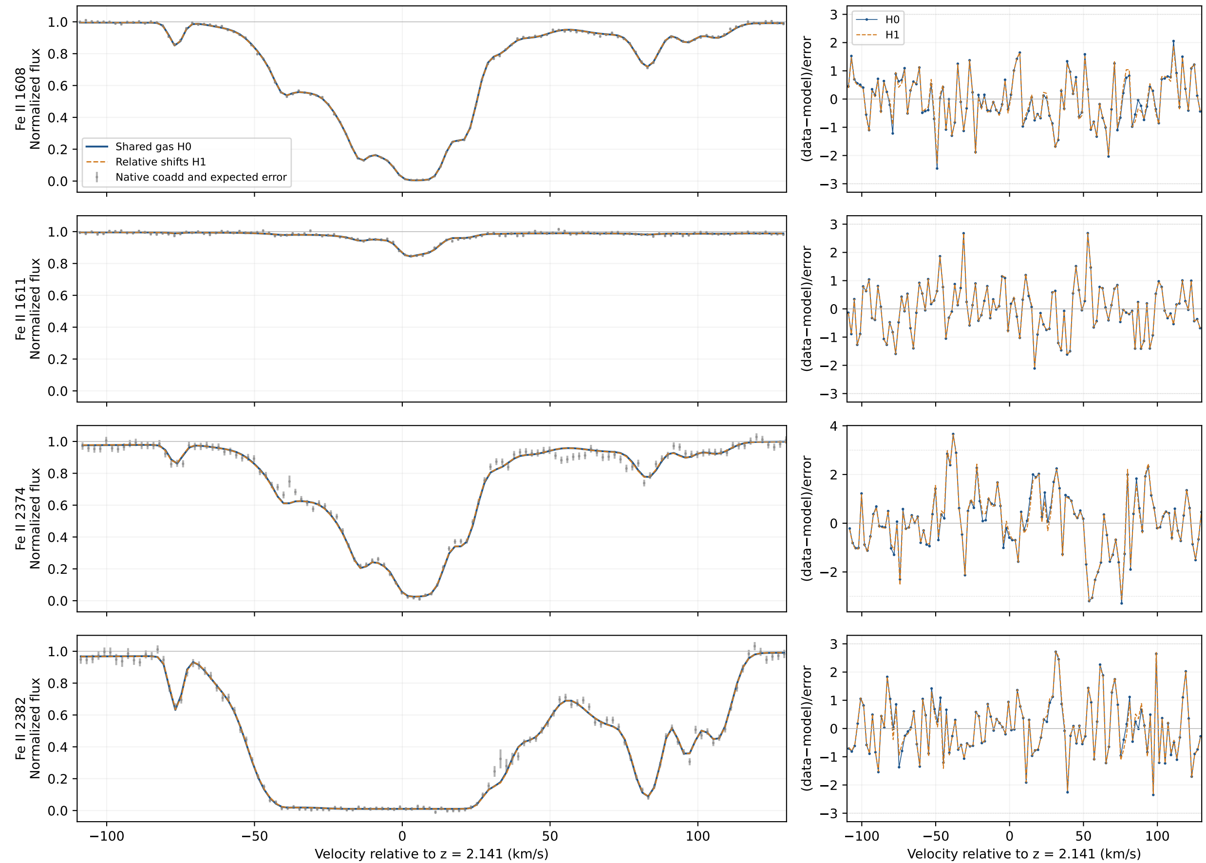
J053007–250329: 16 shared Voigt components, 480 native pixels H0 \chi^2 / nominal dof = 482.30 / 416; conditional \Delta\chi^2 = 4.18 for 3 additional shifts
