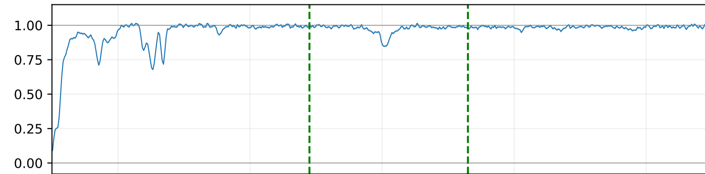
Fe II 1611
