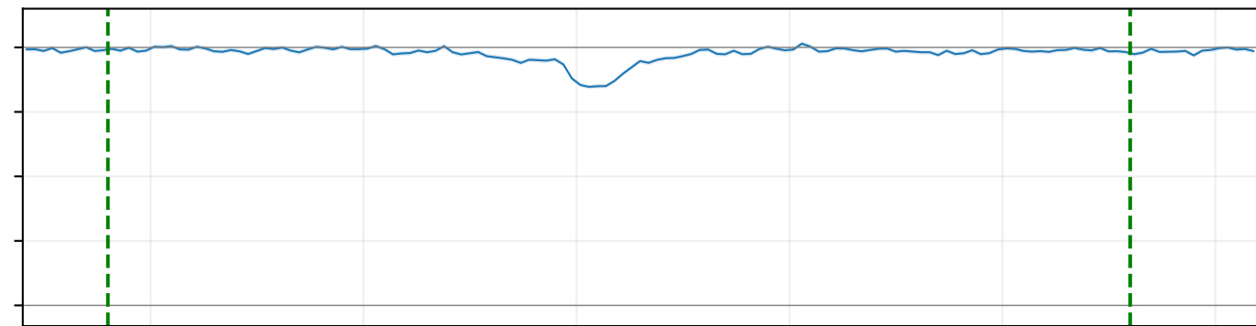
Fe II 1611
