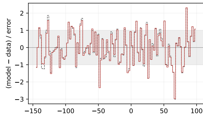
J064326–504112 failed-primary diagnostic: shifts do not repair weak 1611 residuals
