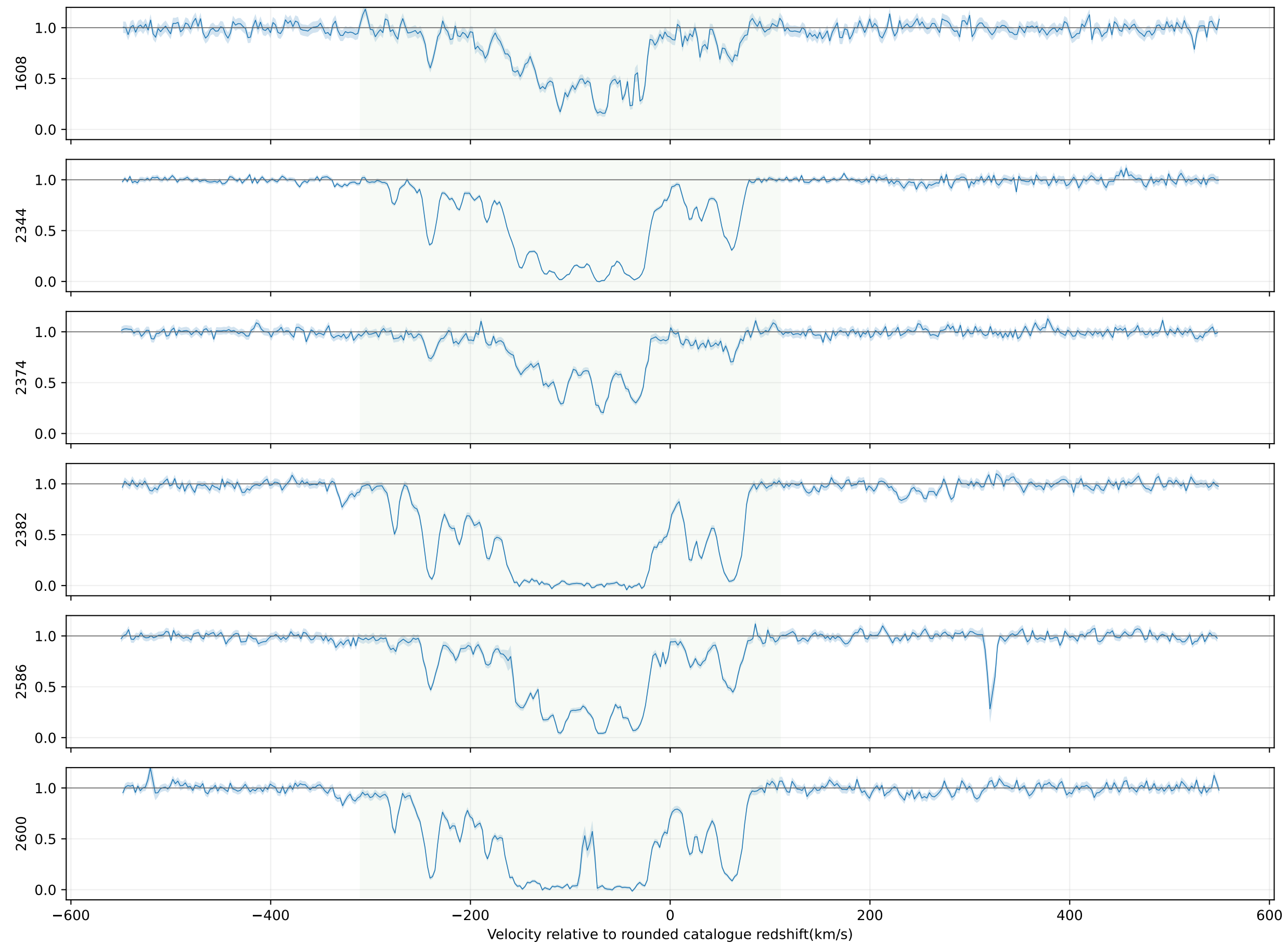
J225719-100104 z1.836: pre-fit selection; shaded common window
