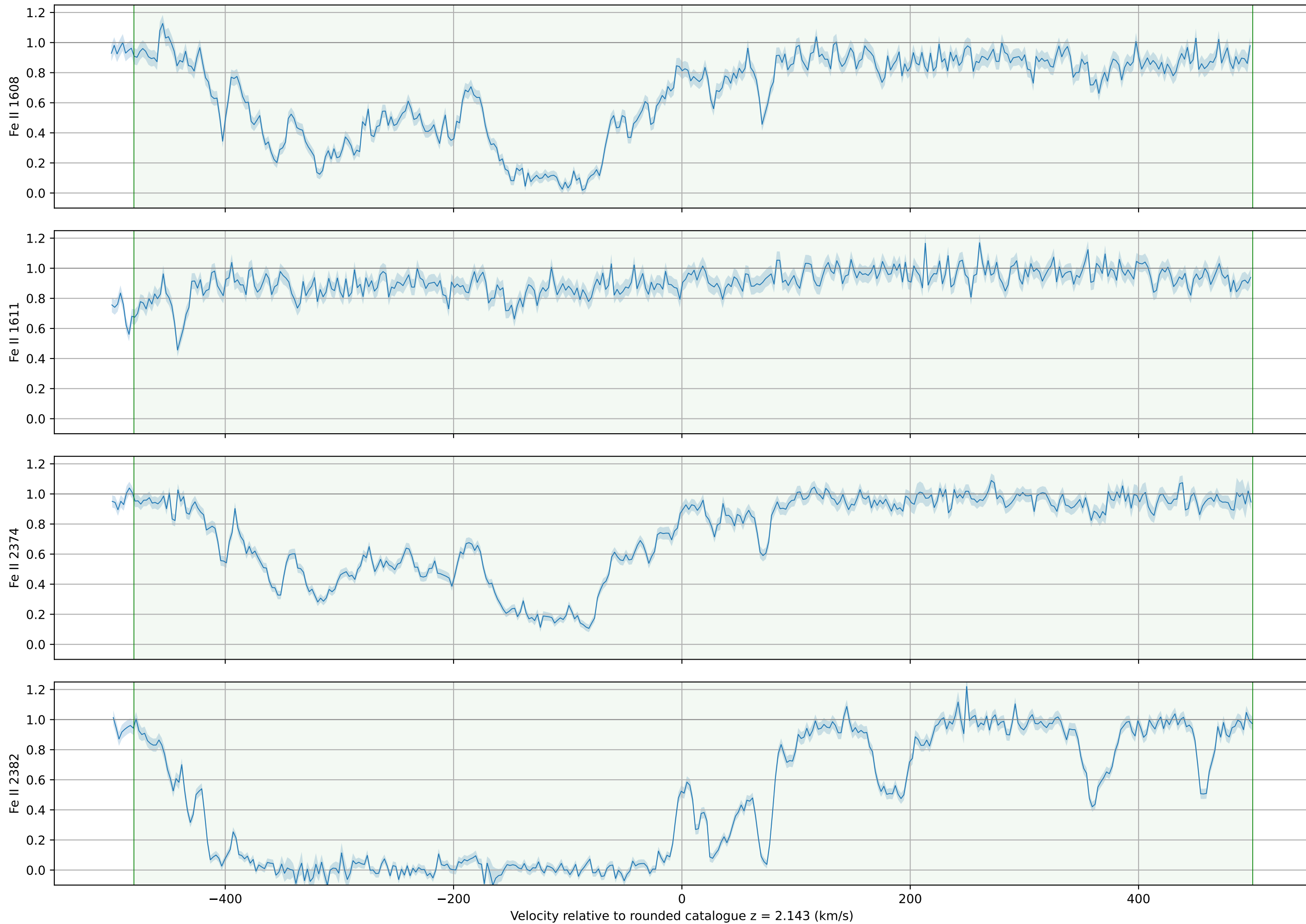
J233156–090802: expanded-complex selection inspected before shift fitting; green interval [−480, +500] km/s
