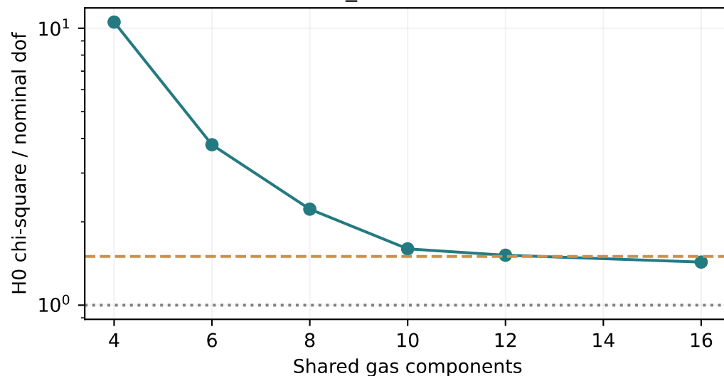
J064326-504112 z_{\text{abs}}=2.659
