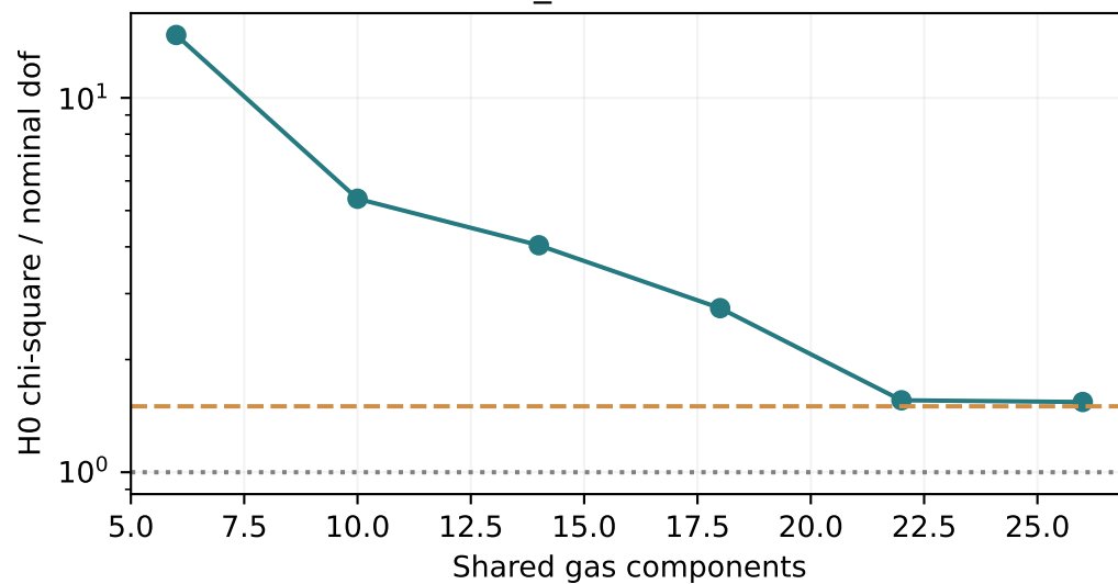
J233156-090802 z_{\text{abs}}=2.143
