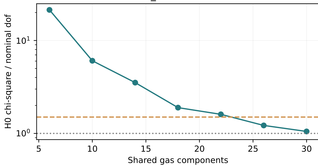
J225719-100104 z_{\text{abs}}=1.836
