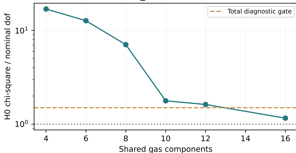
J053007-250329 z_{\text{abs}}=2.141
