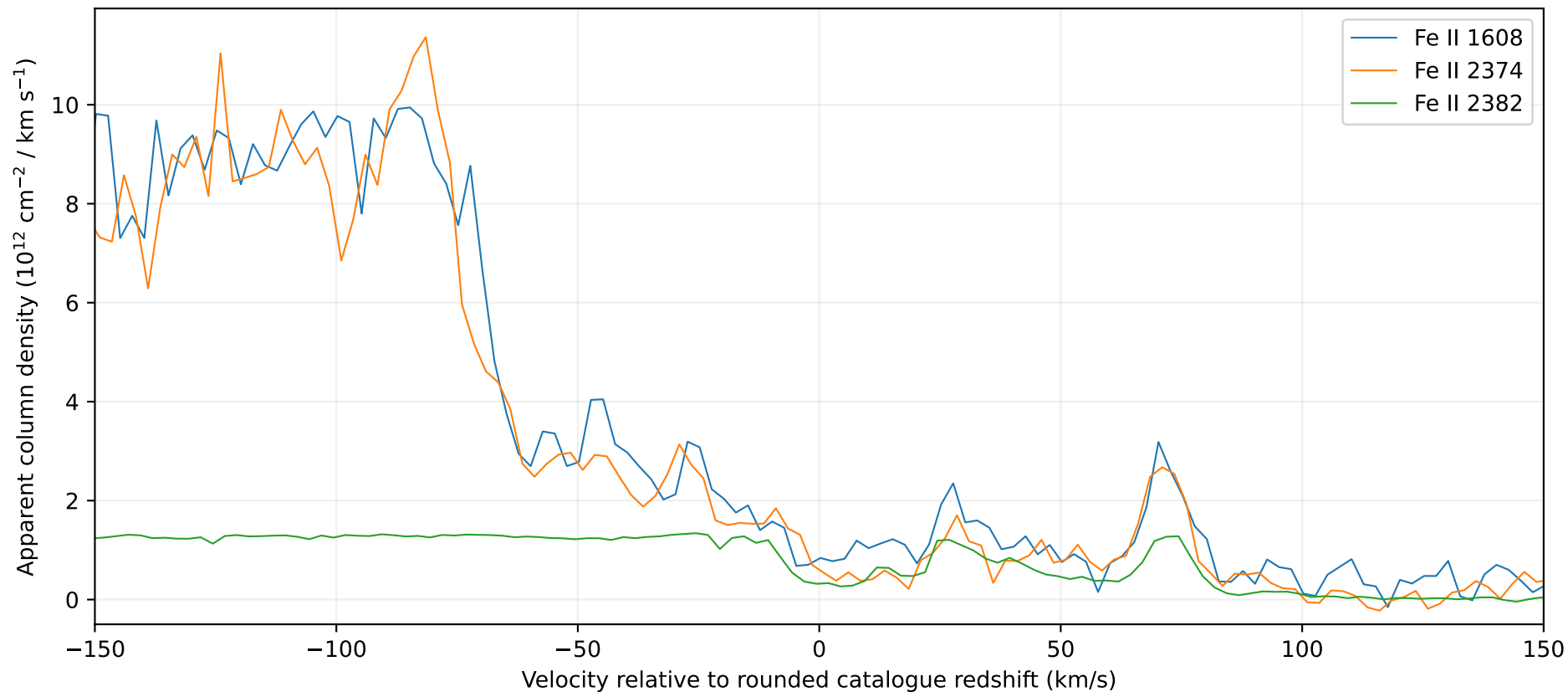
J233156-090802, z_{\text{abs}}=2.143 : AOD consistency diagnostic Low flux uses a 3-error floor; saturation, blends and LSF remain unresolved
