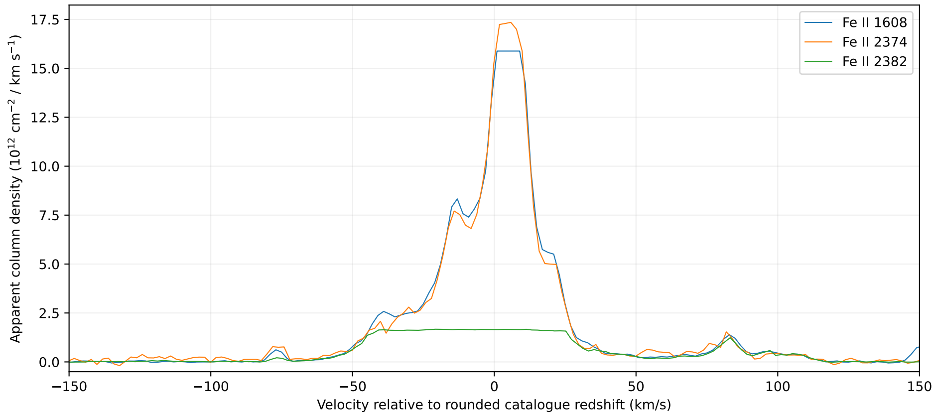
J053007-250329, z_{\text{abs}}=2.141 : AOD consistency diagnostic Low flux uses a 3-error floor; saturation, blends and LSF remain unresolved
