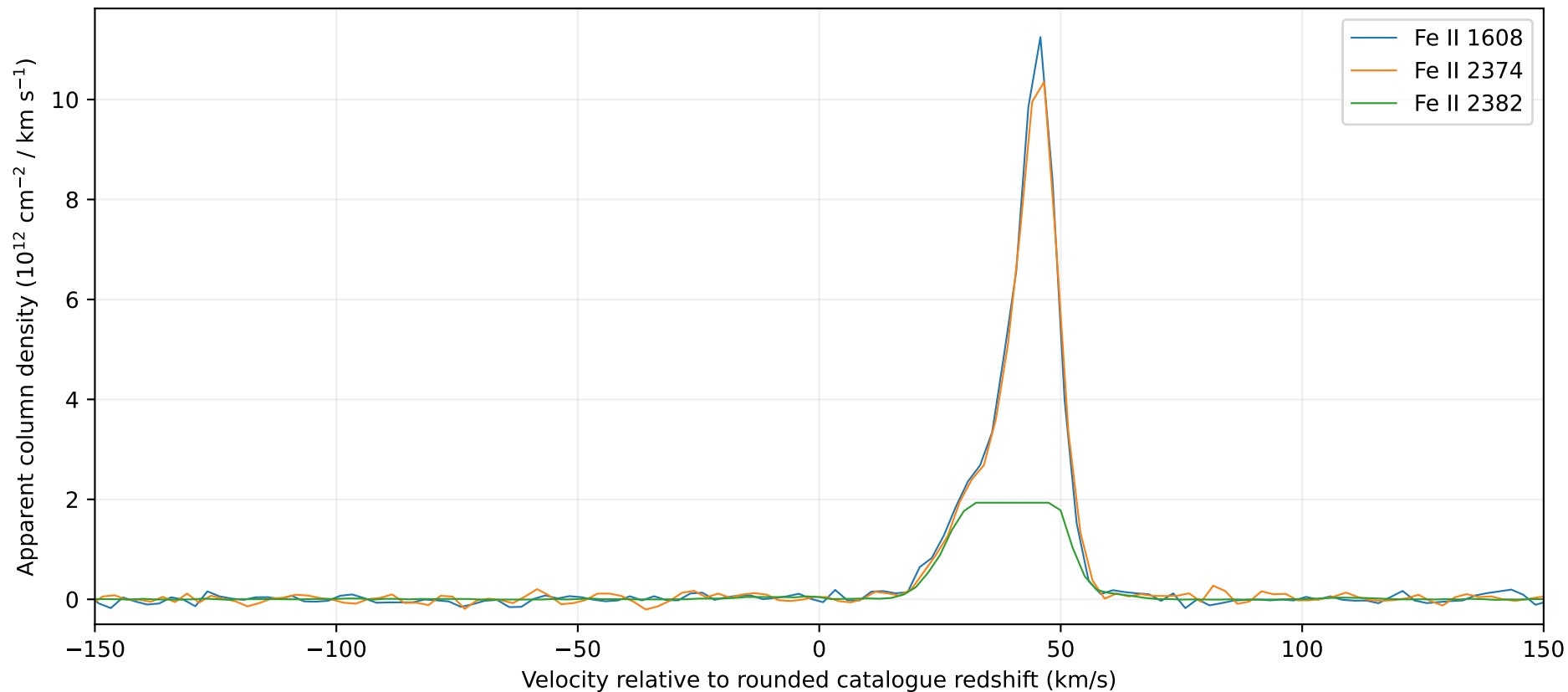
J004131-493611, z_{\text{abs}}=2.248 : AOD consistency diagnostic Low flux uses a 3-error floor; saturation, blends and LSF remain unresolved
