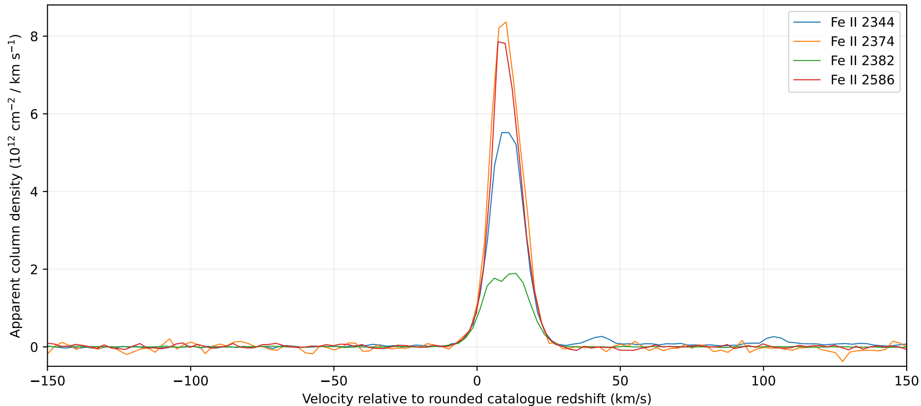
J232128-105122, z_{\text{abs}}=1.629 : AOD consistency diagnostic Low flux uses a 3-error floor; saturation, blends and LSF remain unresolved
