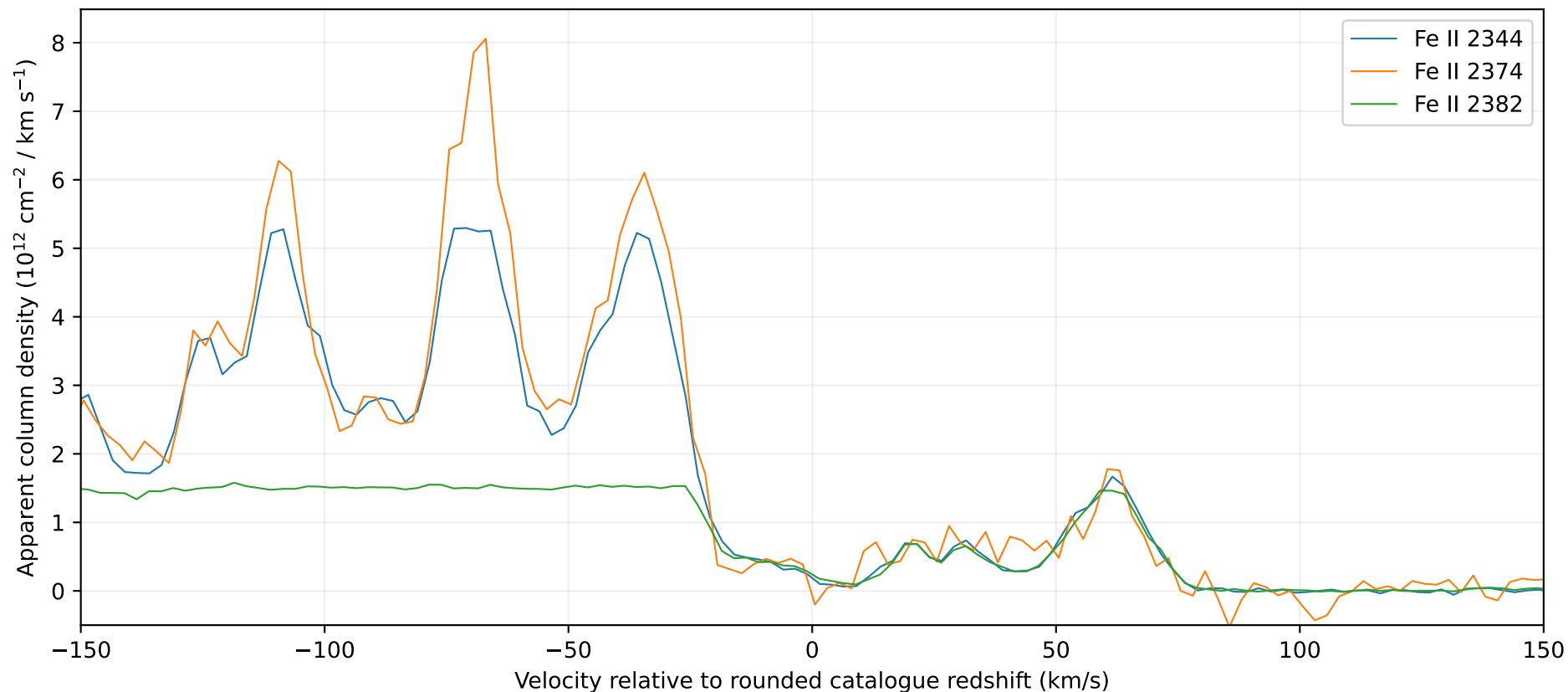
J225719-100104, z_{\text{abs}}=1.836 : AOD consistency diagnostic Low flux uses a 3-error floor; saturation, blends and LSF remain unresolved
