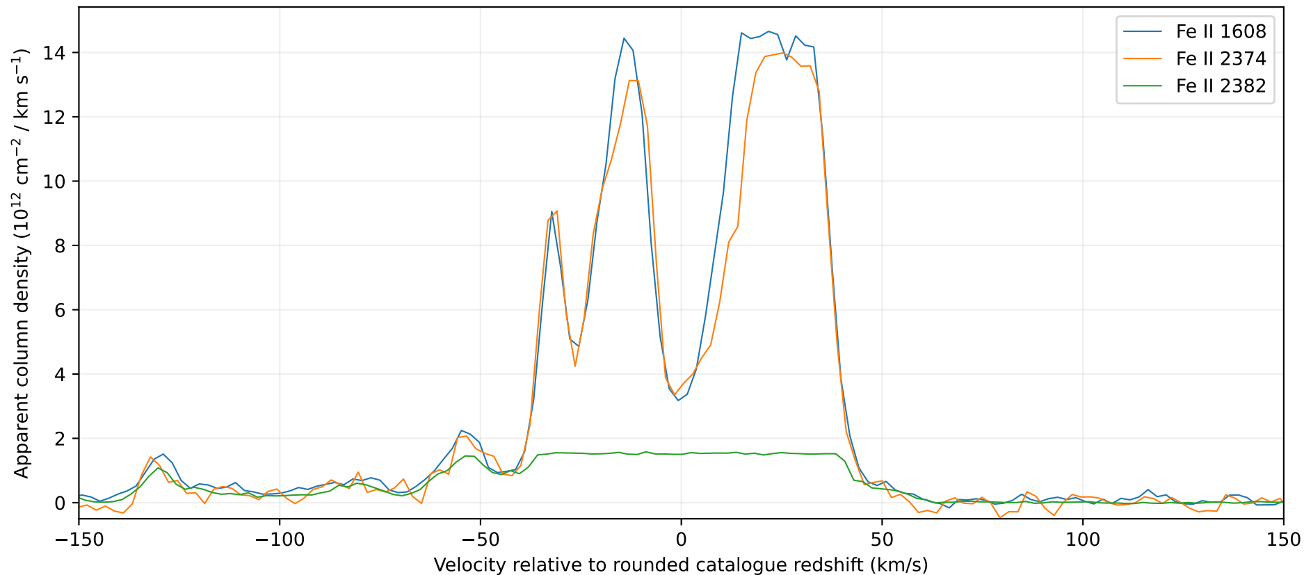
J064326-504112, z_{\text{abs}}=2.659 : AOD consistency diagnostic Low flux uses a 3-error floor; saturation, blends and LSF remain unresolved
