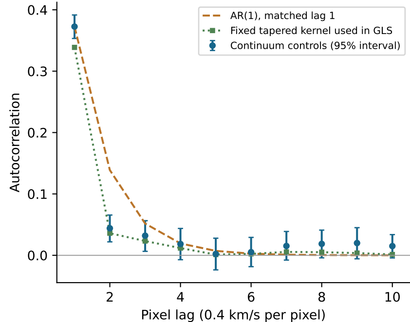
25 disjoint continuum intervals / 13,750 pixels
