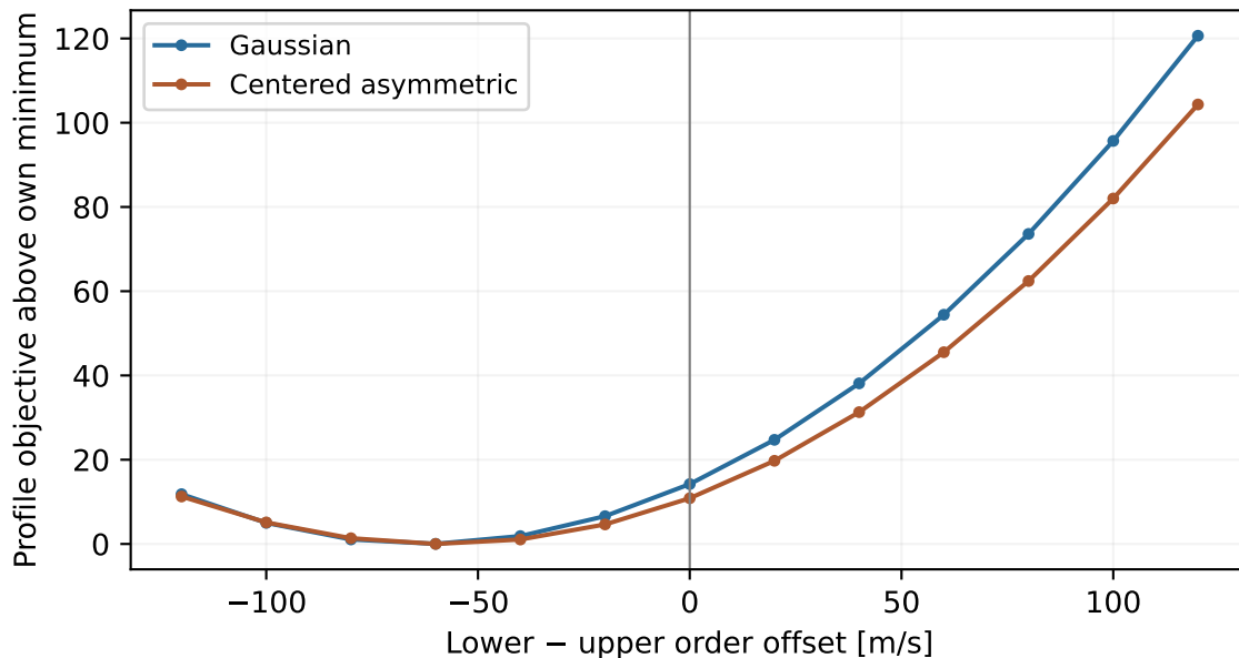
Fe II 2382: conditional offset profiles
