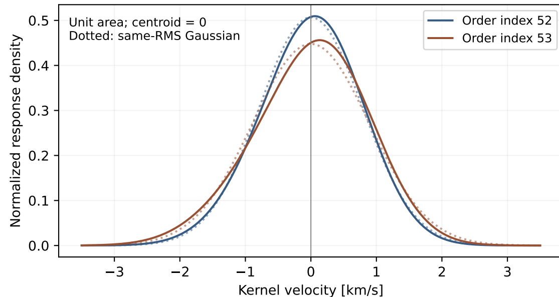
2018 response transferred to 2019-2020
