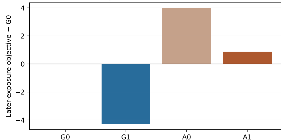
2018 response transferred to 2019-2020
