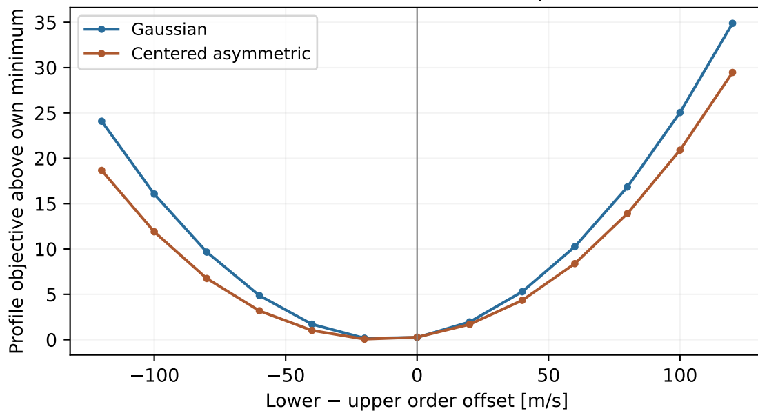
Fe II 2382: conditional offset profiles
