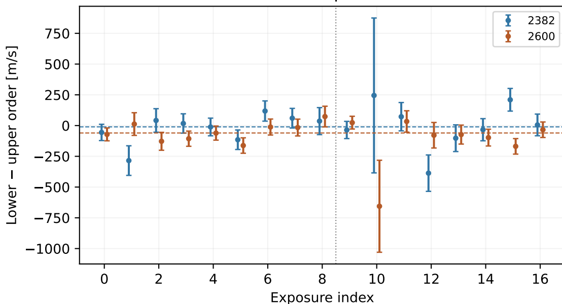
Leave-one-exposure-out stability
