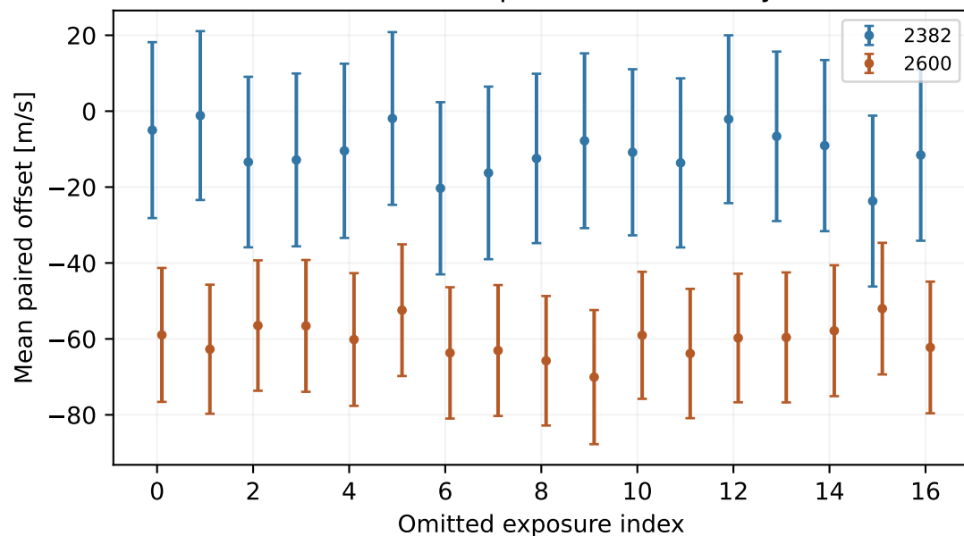
Leave-one-exposure-out stability
