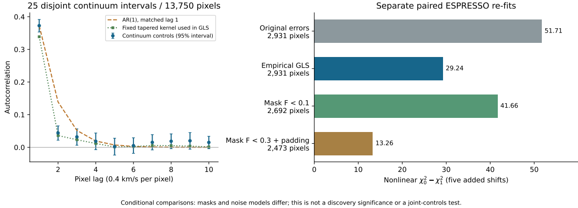
FIG. 8. Continuum controls and subsequent nonlinear sensitivity tests. Left: the measured pixel autocorrelation, interval-resampling uncertainty, and the AR(1) and tapered empirical prescriptions. Right: improvements from adding the same five relative shifts in the original ESPRESSO comparison, the covariance re-fit and the two frozen core-mask re-fits. The covariance and masking changes are tested separately. These comparisons share the underlying observations and are not independent detections.
