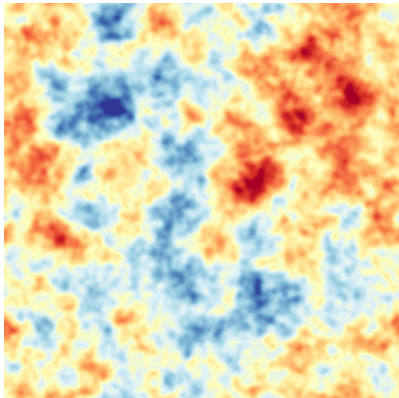
(c) GRF ( \Lambda CDM spectrum) skew=+0.03, kurt=-0.10
