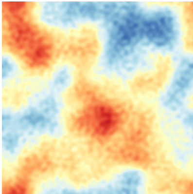
(b) GRF (matched spectrum) skew=-0.04, kurt=-0.60
