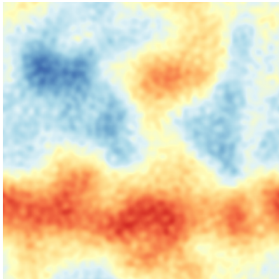
(a) DSC symplectic skew=+0.22, kurt=-0.75
