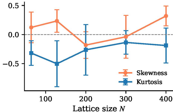
(a) Gaussianity convergence
