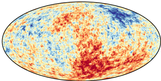
(a) DSC full-sky CMB (3D \rightarrow Mollweide)
