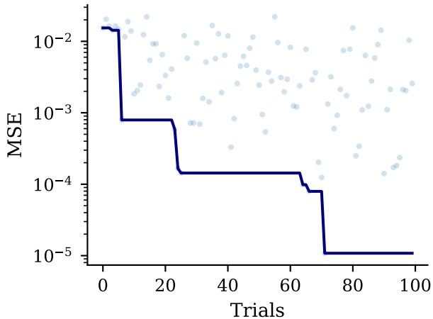
(a) Optimization convergence
