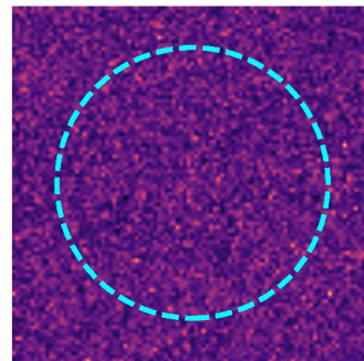
(c) 3D cosmic web
