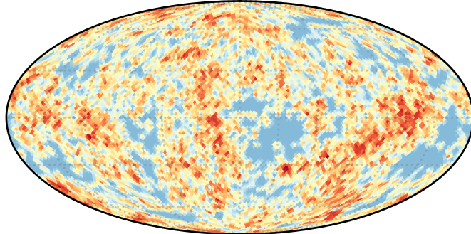
(b) DSC inverse reconstruction
