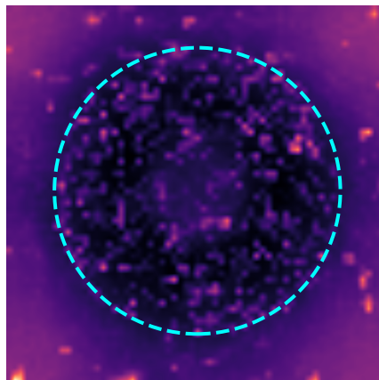
(c) Inferred 3D cosmic web ( 64^3 )
