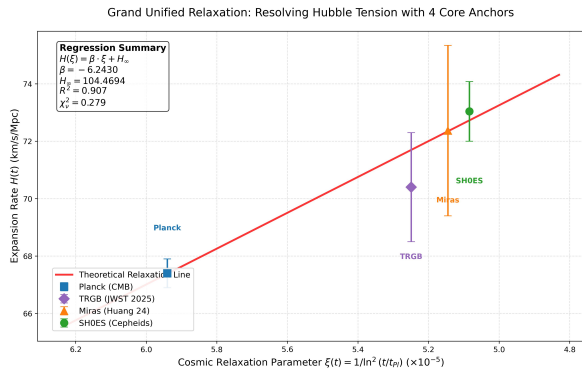
Figure 5: Four H_0 anchors fit by the DSC relaxation law H(t) = H_\infty + \beta/\ln^2(t/t_P) . R^2 = 0.907 , reduced \chi^2 = 0.28 . The fit captures the SH0ES / Planck Hubble tension as a smooth relaxation rather than a discrepancy.
