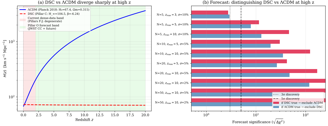
Figure 7: Pillar O: forecast falsifiability of the 1/\ln^2(t) ansatz at high redshift. (a) The DSC and \Lambda CDM Hubble curves diverge sharply at z > 2 ; current dense-data tests (Pillars F–J, z < 2 ) sit in the near-degenerate band, while the forecast band z \in [2, 20] is where future cosmic chronometers can decisively discriminate. (b) Forecast significance ( \sqrt{\Delta\chi^2} ) under various survey configurations. Even a 5-point survey at z_{\text{max}} = 5 with 10% precision suffices for \sim 11\sigma discrimination.
