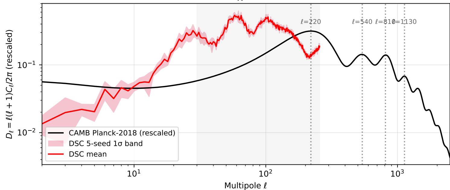
(a) DSC vs CAMB Planck-2018: \chi^2/\text{dof} = 80.41 (band \ell \in [30, 256] )
