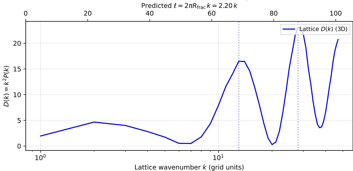
(b) Lattice k -peaks vs Planck multipoles
