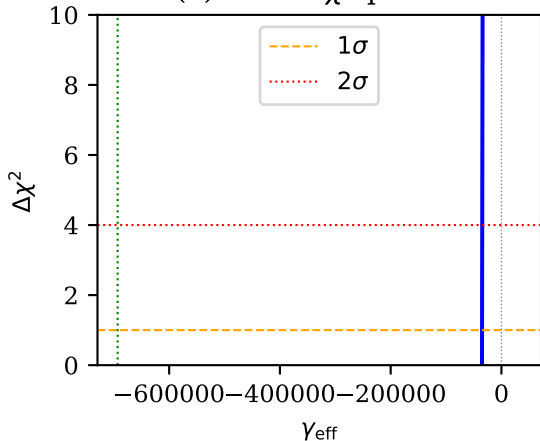
(c) H(z)
