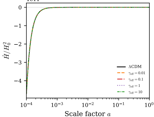
(e) Stability: \dot{H} < 0 always
