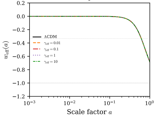
(f) Effective equation of state
