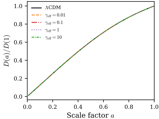
(c) Linear growth factor
