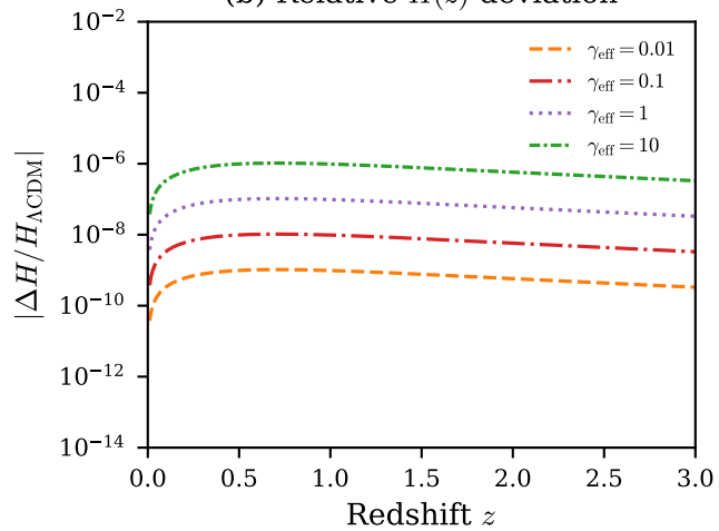
(b) Relative H(z) deviation
