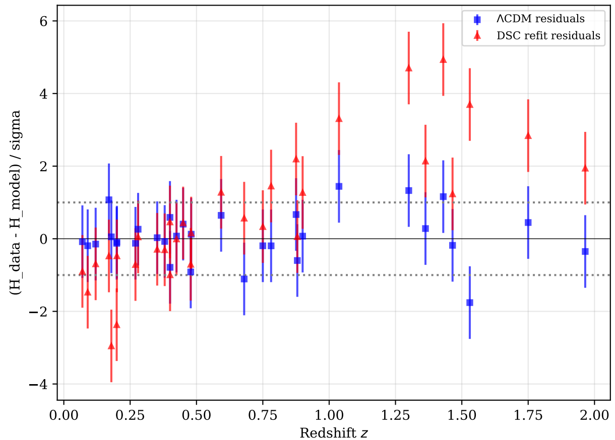
(b) Pull residuals
