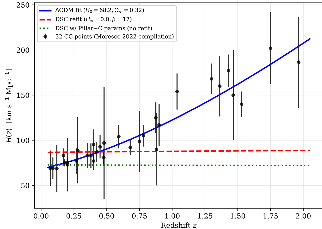
(a) Cosmic chronometer H(z) : 32 points
