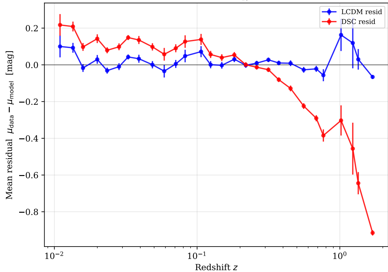
(b) Binned residuals ( \Delta\chi^2 = +617.1 )
