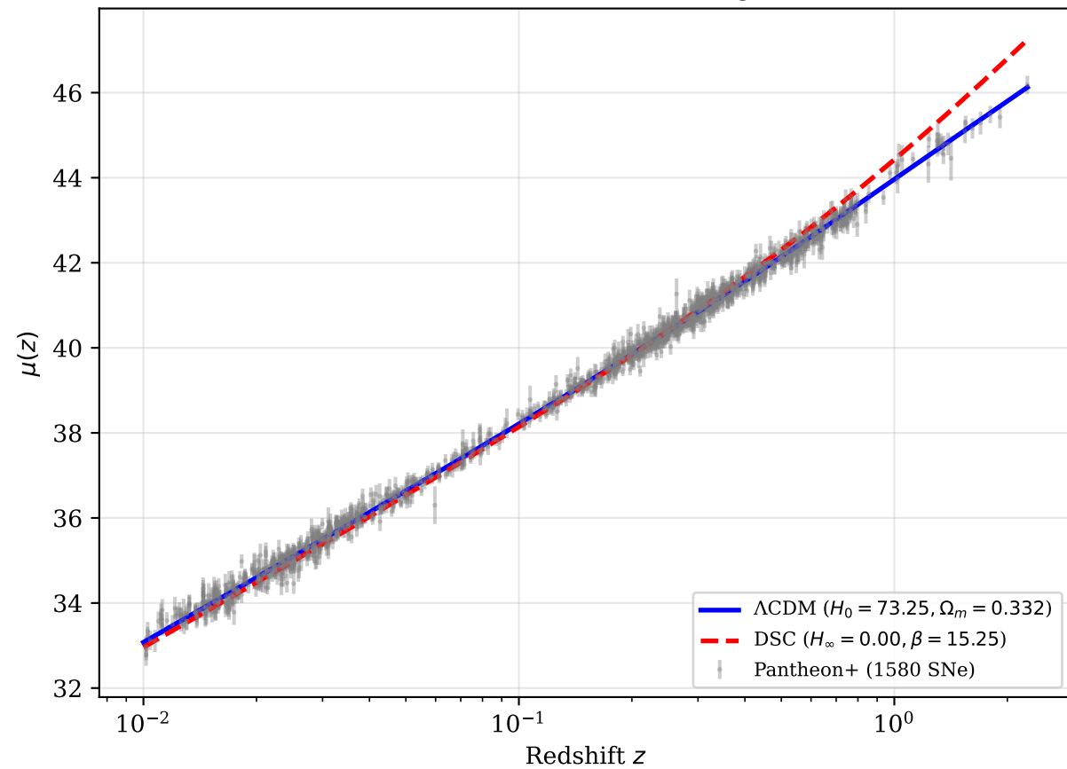
(a) Pantheon+ Hubble diagram
