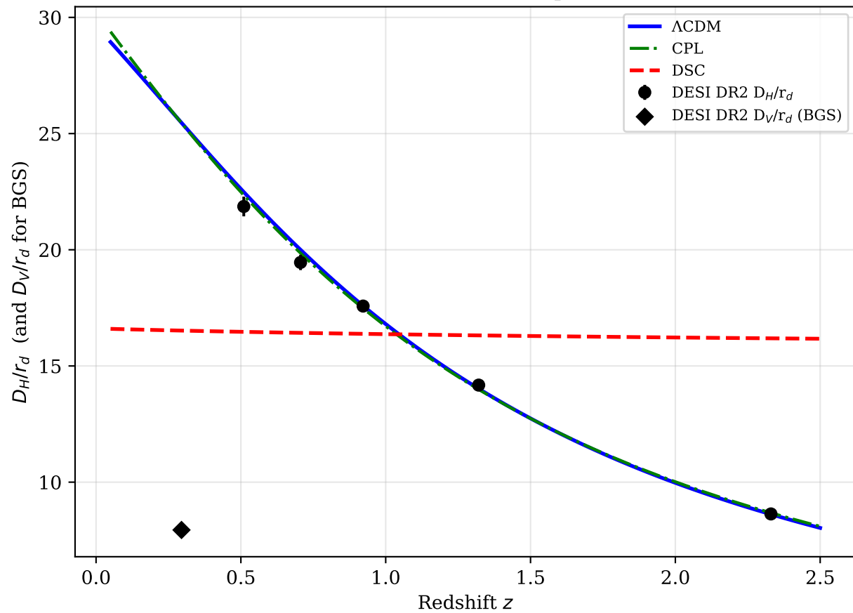
(b) Radial BAO + isotropic BGS
