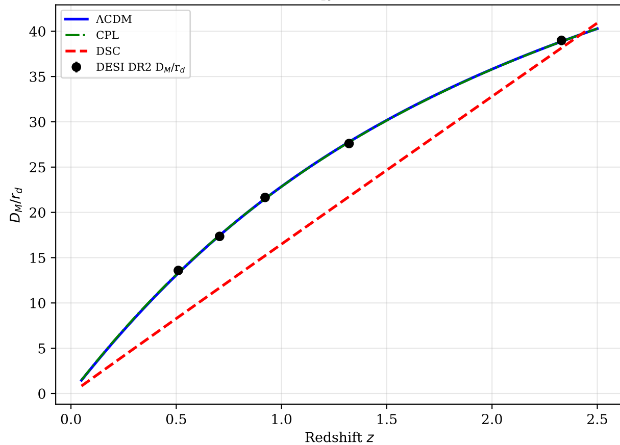
(a) Transverse BAO ( \Delta\chi^2(\text{DSC}-\Lambda\text{CDM})=+14026.3 )
