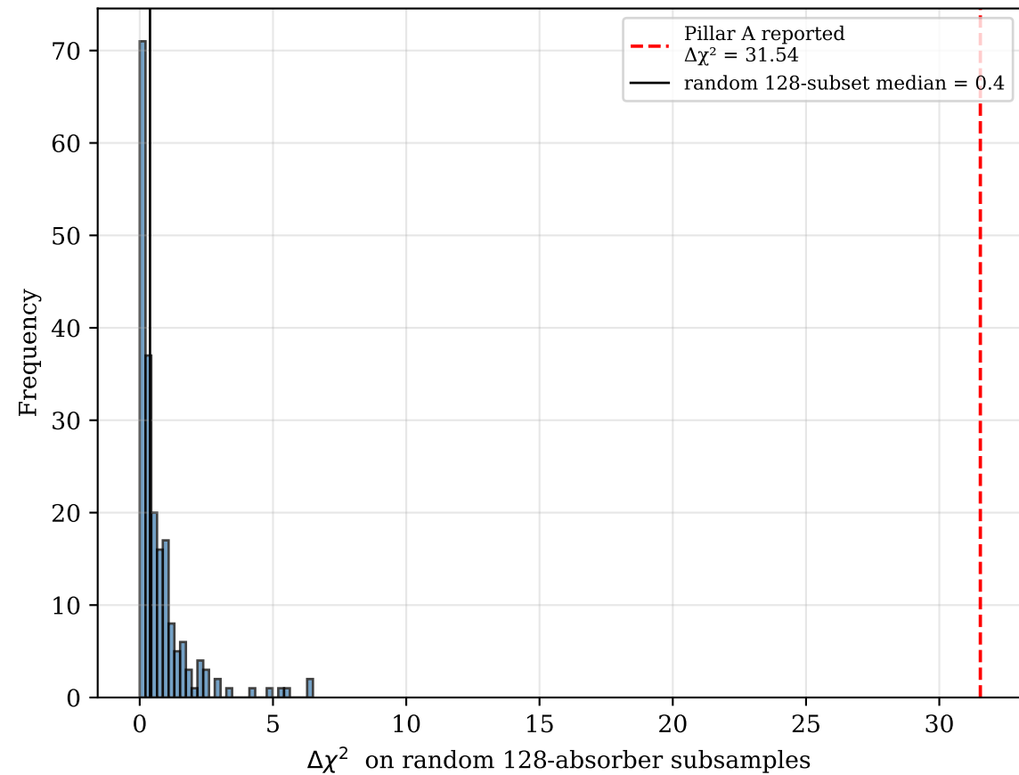
(b) 200 random 128-subset trials
