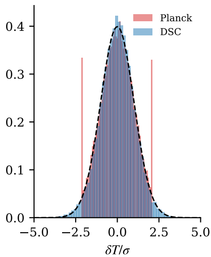
(e) Pixel distribution
