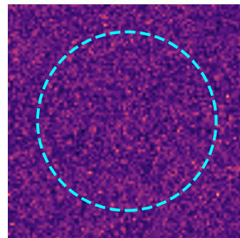
(c) 3D cosmic web
