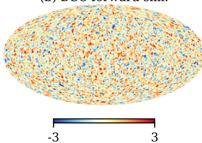
(b) DSC forward sim.
