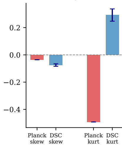
(f) Gaussianity comparison
