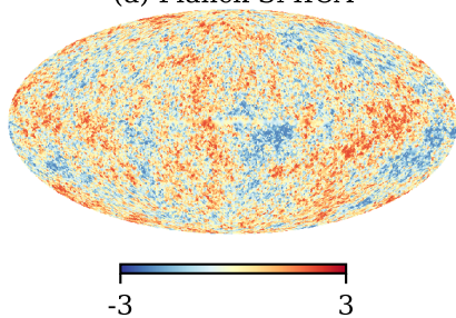
(a) Planck SMICA
