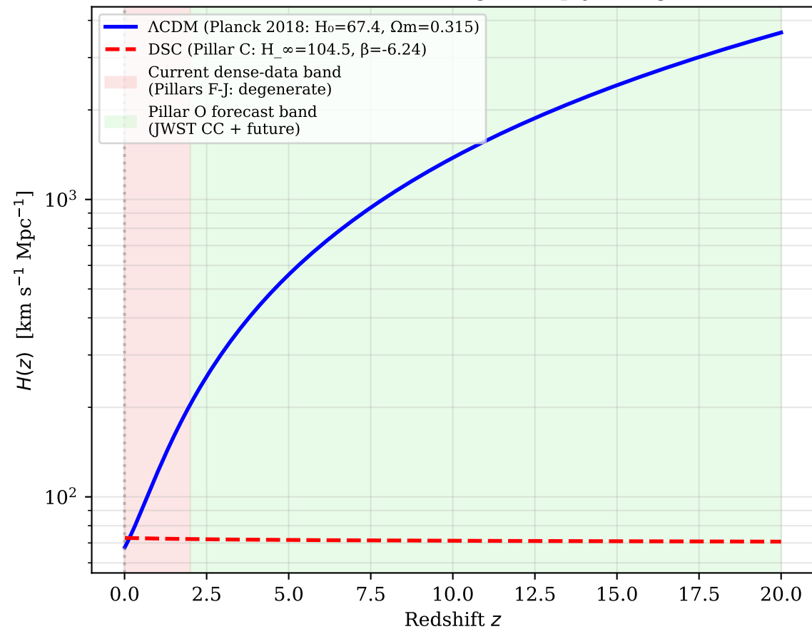
(a) DSC vs \Lambda CDM diverge sharply at high z
