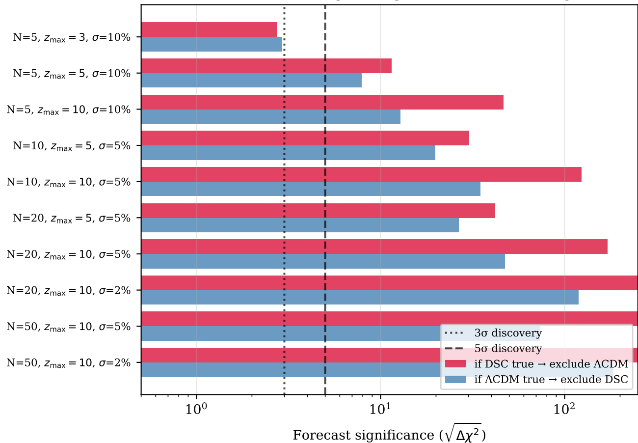
(b) Forecast: distinguishing DSC vs \Lambda CDM at high z
