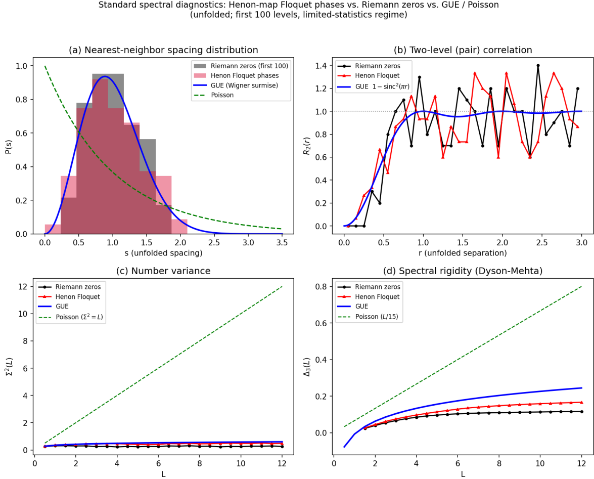
Figure 7: Standard local spectral diagnostics (unfolded; first 100 levels) for the Hénon Floquet eigenphases (red) and the true Riemann zeros (black), against GUE (blue) and Poisson (green). (a) Nearest-neighbor spacing distribution: both show level repulsion (suppression at s \rightarrow 0 ) consistent with GUE, not Poisson. (b) Two-level correlation R_2(r) , showing the GUE correlation hole. (c) Number variance \Sigma^2(L) and (d) spectral rigidity \Delta_3(L) , both following the logarithmic GUE curves rather than the linear Poisson behavior. Generated by 8-spectral_diagnostics.py .
