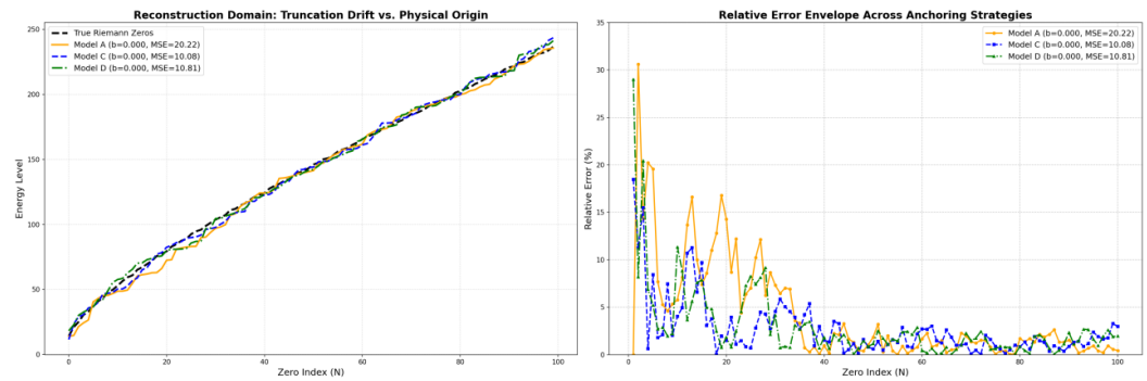
Figure 4. Reconstruction Domains and Anchoring Strategies: A Comparative Analysis of Models A, C, and D. This figure shows single-run experiments with fixed predetermined values of k (Model A: k \approx 7.429 , Model C: k \approx 8.070 , Model D: k \approx 8.783 ) to visually illustrate the qualitative behavior of different anchoring strategies and their residual envelopes over 100 orders. These fixed-parameter experiments differ from the global optimization protocol used in Table 1, where k is itself the variable being optimized to minimize MSE; the numerical values of k therefore differ between the two experimental setups and should not be directly compared. Model A (Orange / Single-Point Anchoring): Utilizes solely the first zero as the absolute physical baseline. While strictly aligning the ground state, it accumulates the largest macroscopic divergence over 100 orders (MSE \approx 20.22 ). Model C (Blue / Forced Origin Scaling): Represents a global least-squares fit constrained to the origin ( b = 0 ) within the single-sided positive spectrum, which suppresses error divergence relative to Model A, yielding a lower mean squared error (MSE \approx 10.08 ). Model D (Green / Conjugate Full Spectrum Free Fit): Uses both positive and negative eigenphases. Because the regression data are symmetric under (\theta, \gamma) \rightarrow (-\theta, -\gamma) , the least-squares intercept is algebraically forced to b = 0.000 (Section 3.2.2); the fitted slope and the resulting residual envelope (MSE \approx 10.81 ) are the model-specific numerical content of this comparison.
