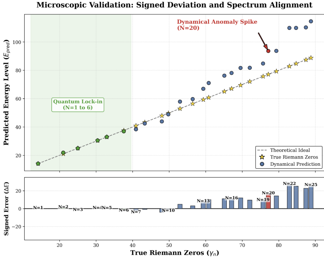
Figure 2. Microscopic comparison of the dynamical eigen-spectrum and the N=20 residual feature.
