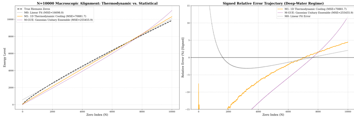
Figure 7. Ultra-Macroscopic Spectral Alignment (N=10,000): Thermodynamic Cooling vs. Statistical Baselines. M-GUE (Purple Dashed / Gaussian Unitary Ensemble): The pure Random Matrix Theory baseline shows a large structural divergence (MSE \approx 255455.9 ) in this counting-function comparison. This illustrates that without a deterministic cooling mechanism, a single globally scaled Wigner’s Semicircle spectrum does not capture the macroscopic logarithmic density of the Riemann manifold. M1 (Orange Solid / 1D Thermodynamic Cooling): The 1D non-autonomous dynamical model ( k_1 \approx 13.431 ) paces the true Riemann zeros, tracking both the sensitive low-frequency ground states and the high-order high-frequency states.
