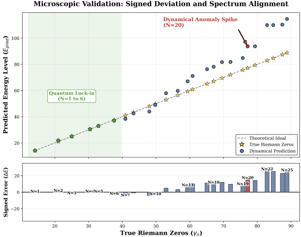
Figure 2. Figure 2. Microscopic empirical validation of the dynamical eigen-spectrum and the emergence of the N=20 resonance anomaly. (Top) The alignment trajectory of the dynamical predicted energy levels ( E_{pred} , colored dots) and the true Riemann zeros ( \gamma_n , golden stars) under the critical numerical discrete scale \epsilon=0.001916 . In the low-frequency limit ( N=1 to 6, green shaded area), the system achieves high-fidelity “Quantum Lock-in,” verifying the accuracy of the ground state linear homomorphic mapping. (Bottom) Actual dynamical residual distribution with signs ( \Delta E=E_{pred}-\gamma_n ). Despite being constrained by nonlinear state density, causing the system to exhibit natural systematic phase drift at higher energy levels, when evolving to N=20 , the predicted spectrum spontaneously excites an extremely steep, isolated structural breaking—a dynamical anomaly spike (marked in red). This nonlinear resonance anomaly, “blind-box emerged” from a purely numerical computing engine under finite precision, achieves a notable homomorphic benchmarking in both position and mutational tendency with the inexplicable massive measurement error bars encountered at the same energy level in recent physical ion-trap quantum simulation experiments.
