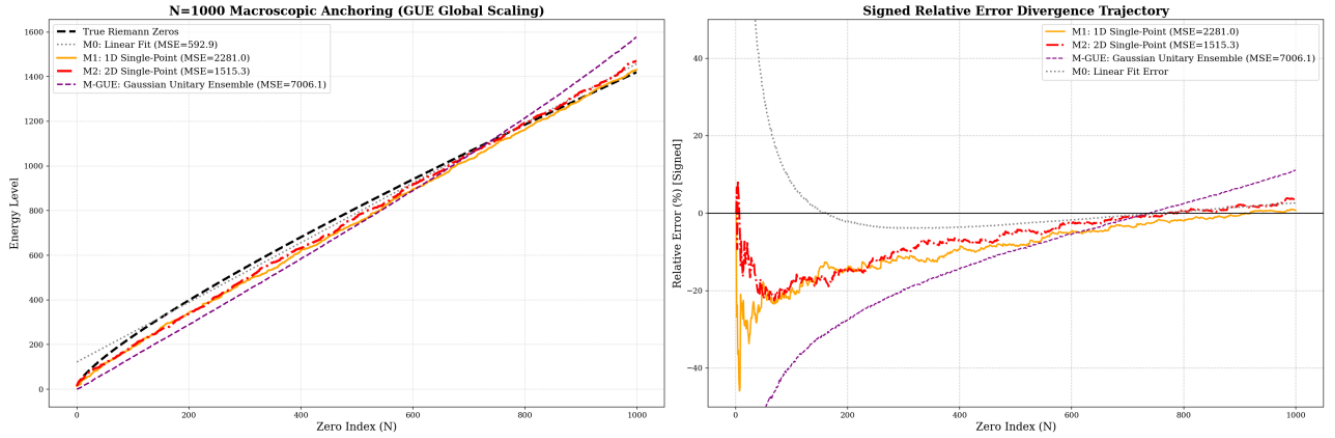
Figure 6. Figure 6: Macroscopic Spectral Alignment and RMT Ablation: Deterministic Cooling vs. Wigner's Semicircle. Model M-GUE (Purple Dashed / Gaussian Unitary Ensemble): Serving as the microscopic statistical baseline, the GUE matrix exhibits severe non-linear macroscopic divergence (right panel, MSE \approx 7006.1 ) even under optimal Global Least-Squares Scaling. This explicitly exposes that pure random matrices, governed by Wigner's Semicircle Law, inherently lack the critical macroscopic logarithmic density features required to approximate the Riemann manifold. Models M1 & M2 (Orange & Red / Non-autonomous Dynamics): Represent the 1D and 2D dynamic prediction models proposed in this work. Under the extremely rigorous constraint of Single-Point Anchoring (utilizing solely the first zero), M1 and M2 demonstrate notable macroscopic topological rigidity. Specifically, the 2D model (red line) with the running coupling constant not only eliminates systematic parabolic drift over a span of N=1000 orders, but also suppresses the global residual to a minimal level ( MSE \approx 1515.3 ).
