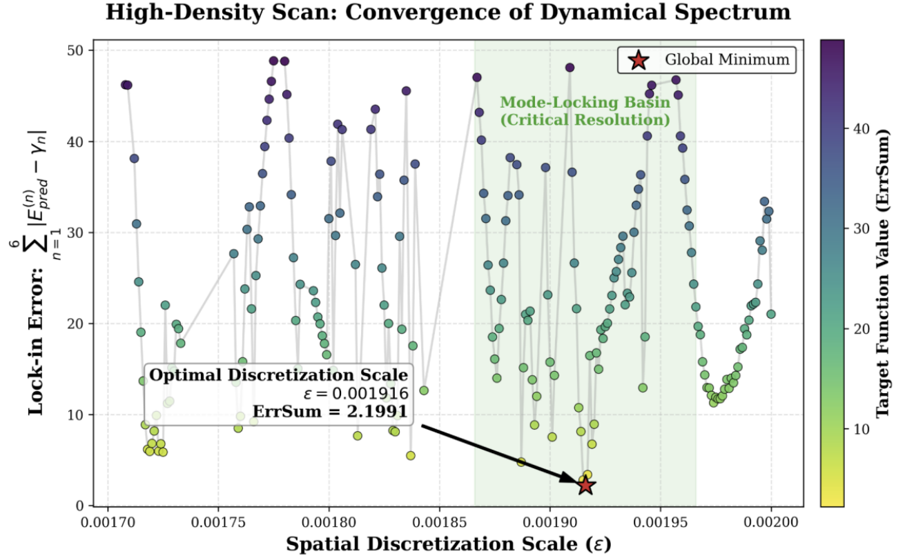
Figure 1. Figure 1. High-density parameter scanning and the emergence of mode-locking under the critical discrete scale. The scatter plot displays the trajectory of the objective function ErrSum (the sum of absolute deviations of the first 6 eigen-energy levels) varying with the spatial discretization scale \epsilon . Within the “mode-locking basin” (green shaded area) determined by the broadband coarse scan, the spectral deviation exhibits strong non-linear oscillation. When \epsilon advances to the global minimum 0.001916 (red star, ErrSum=2.1991), the system undergoes an extremely steep numerical phase transition. This critical point signifies that the continuous Fokker-Planck numerical diffusion has precisely and closely neutralized the discrete spatial truncation error, allowing the system’s pure dynamical eigen-spectrum to emerge.
