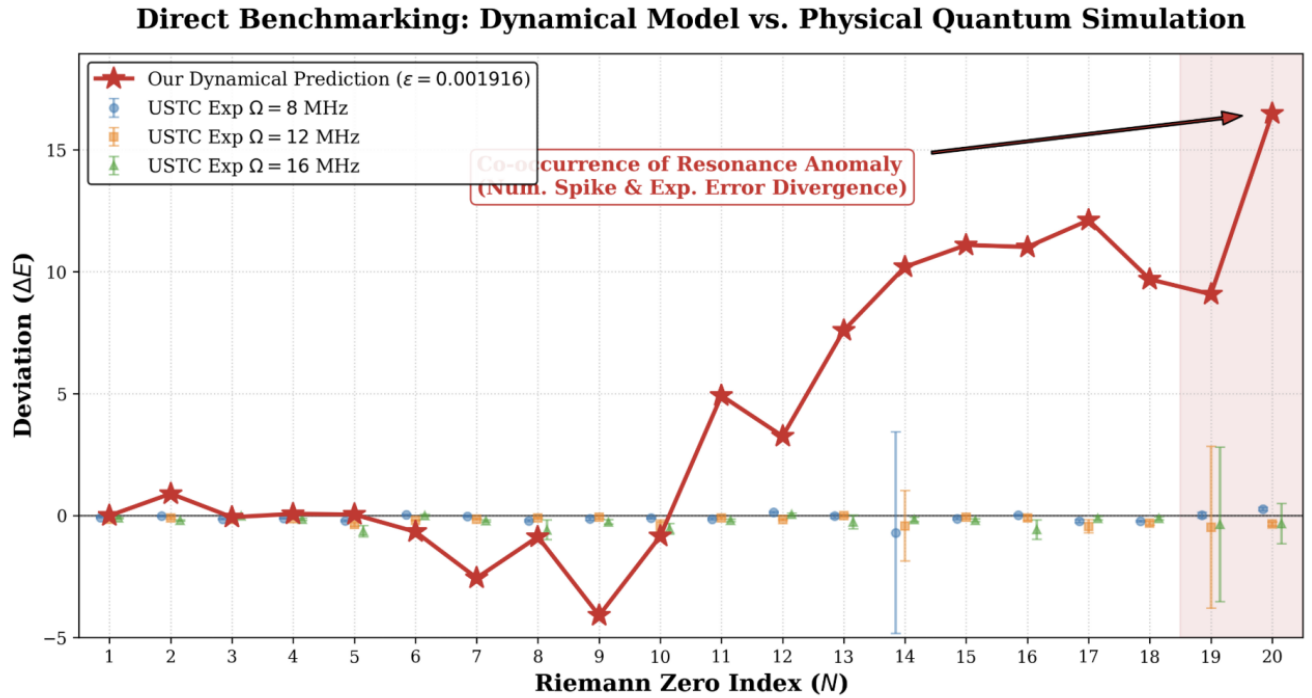
Figure 3. Figure 3. Direct Benchmarking: Back-to-back comparison of the dynamical numerical model and physical quantum simulation. Direct comparison of our numerical prediction residuals (red star line) with USTC physical experimental data (ion-trap quantum simulation under different trap frequencies \Omega ). In the N < 19 region, the numerical model successfully captured the near-zero fluctuation baseline of the physical system. Crucially, at N = 19 \sim 20 , the numerical computation's “anomaly spike” and the severe divergence of experimental measurement uncertainty (red shaded area) completely align in position and qualitative characteristics. This high degree of commonality provides strong evidence that “experimental collapse is an intrinsic topological property of finite-precision dynamics rather than random instrumental error.”
