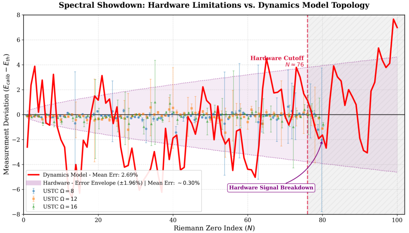
Figure 5. Figure 5: Spectral Showdown: Hardware Limitations vs. Dynamics Model Topology. * Scatter Points and Purple Shading (Quantum Hardware): Displays the actual measurement deviations from the University of Science and Technology of China (USTC) ion-trap quantum hardware. Primarily limited by quantum decoherence effects, the experimental hardware experiences signal breakdown in the N \approx 76-80 band, establishing a physical error envelope restricted to \pm 1.96\% . Red Solid Line (Dynamics Model): Represents the theoretical deviation trajectory derived from 10 billion steps of evolution using the proposed dynamics model (Model C: Single-sided positive spectrum forced origin scaling, k_1=8.070 ). The model's mean error is 2.69%. The model successfully overcomes the hardware's physical limitation boundary, extending deterministic predictions stably to the N=100 order. Notable is the surprising spatial synchronization between the macroscopic oscillation peaks of the theoretical model (red line) and the local error extrema of the quantum hardware (around N \approx 20, 40, 76 ).
