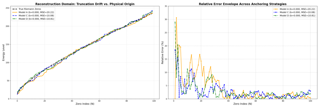
Figure 4. Figure 4: Reconstruction Domains and Anchoring Strategies: A Comparative Analysis of Models A, C, and D. * Model A (Orange / Single-Point Anchoring): Utilizes solely the first zero as the absolute physical baseline ( k \approx 7.429 ). While strictly aligning the ground state, it accumulates the largest macroscopic divergence over 100 orders ( MSE \approx 20.22 ). Model C (Blue / Forced Origin Scaling): Represents the optimal engineering compromise within the single-sided positive spectrum ( k \approx 8.070 ). By applying a global least-squares fit constrained to the origin ( b=0 ), it effectively suppresses error divergence, yielding the lowest global mean squared error ( MSE \approx 10.08 ). Model D (Green / Conjugate Full Spectrum Free Fit): Represents the most complete physical topology ( k \approx 8.783 ). When executing a completely free linear fit incorporating both positive and negative energy states (conjugate spectrum), the system reveals a striking intrinsic symmetry—the intercept spontaneously zeros out ( b=0.000 ). It achieves a highly robust residual envelope ( MSE \approx 10.81 ) without any artificial truncation constraints.
