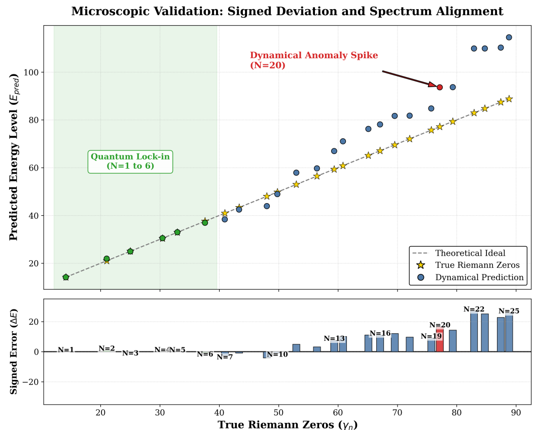
Figure 2. Microscopic comparison of the dynamical eigen-spectrum and the N = 20 residual feature. (Top) The alignment trajectory of the dynamical predicted energy levels ( E_{\text{pred}} , colored dots) and the true Riemann zeros ( \gamma_n , golden stars) under the critical numerical discrete scale \epsilon = 0.001916 . In the low-frequency limit ( N = 1 to 6 , green shaded area), the system achieves close alignment (informally, “lock-in”), consistent with the accuracy of the first-zero-anchored linear rescaling. (Bottom) Actual dynamical residual distribution with signs ( \Delta E = E_{\text{pred}} - \gamma_n ). Constrained by nonlinear state density, the system exhibits systematic phase drift at higher energy levels, and near N = 20 the predicted residuals show a steep, isolated spike (marked in red), which the author compares with a similarly located feature in ion-trap quantum simulation data below (Section 4.1.5).
