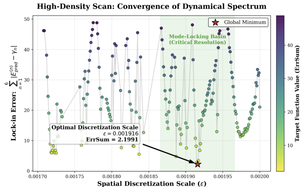
Figure 1. High-density parameter scanning and the emergence of mode-locking under the critical discrete scale. The scatter plot displays the trajectory of the objective function \text{ErrSum} (the sum of absolute deviations of the first 6 eigen-energy levels) varying with the spatial discretization scale \epsilon . Within the “mode-locking basin” (green shaded area) determined by the broadband coarse scan, the spectral deviation exhibits strong non-linear oscillation. When \epsilon advances to the global minimum 0.001916 (red star, \text{ErrSum} = 2.1991 ), the system undergoes a sharp numerical convergence transition. This critical point signifies that the continuous Fokker-Planck numerical diffusion has precisely and closely neutralized the discrete spatial truncation error, allowing the system’s pure dynamical eigen-spectrum to emerge.
