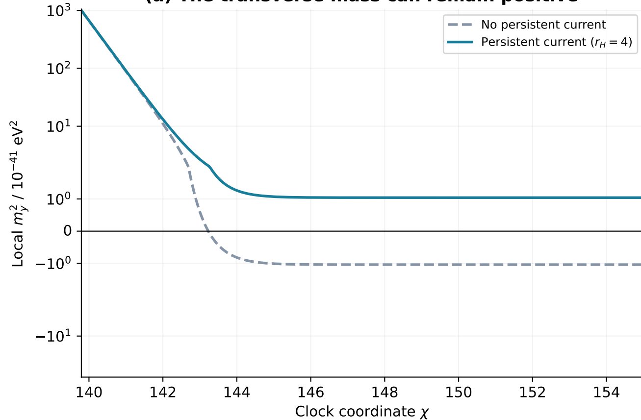
(a) The transverse mass can remain positive
