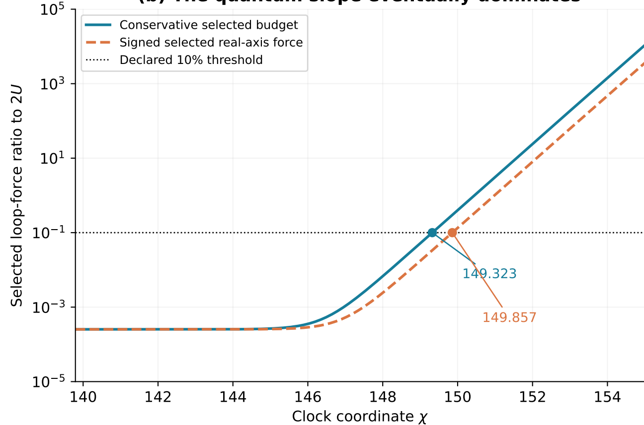
(b) The quantum slope eventually dominates
